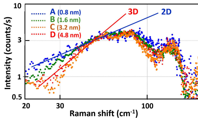
Figure 6. Log-log plot of the VDOS extracted from the Raman data of 4 samples (A to D). The straight lines refer to the Debye approximation (slopes values equal 1 or 2 for dimensionality 2 or 3, respectively).
