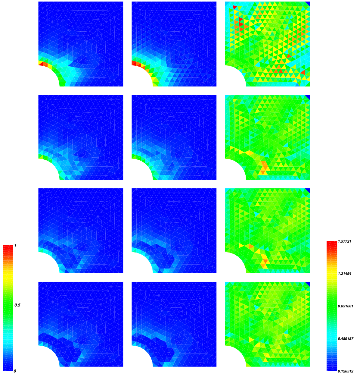
Figure 8: Relative residual errors on uniformly refined patches: residual based error \tilde{\theta}_T (23) - reference error \tilde{\theta}_T^{ref} - normalized error ratio
