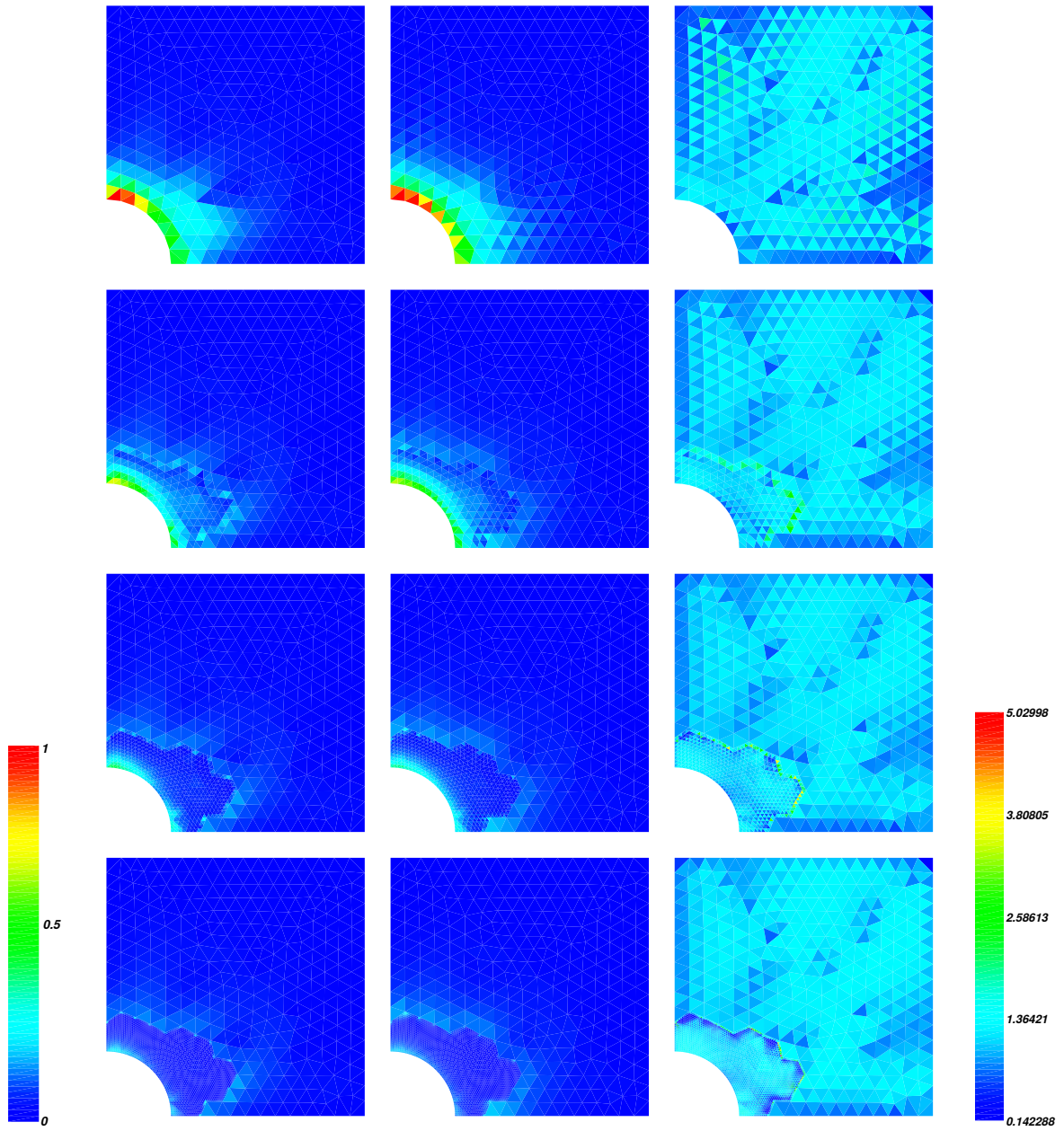
Figure 7: Relative residual errors on uniformly refined patches: residual based error \widehat{\theta}_T (22) - reference error \widehat{\theta}_T^{ref} - normalized error ratio
