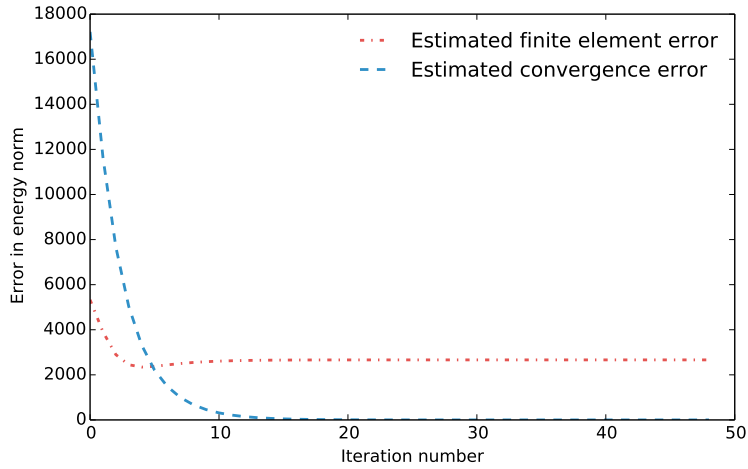
Figure 14: Evolution of the convergence error \Theta_n and the finite elements error \Theta(u_{Hh}^n)
