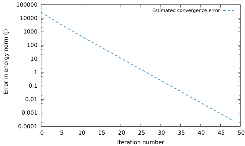
Figure 13: Evolution of the convergence error \Theta_n
