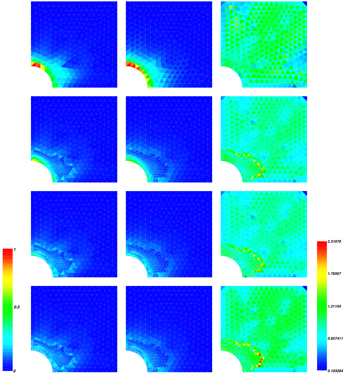
Figure 10: Relative residual errors on non-uniformly refined patches: residual based error \widehat{\theta}_T - reference error \widehat{\theta}_T^{ef} - normalized error ratio
