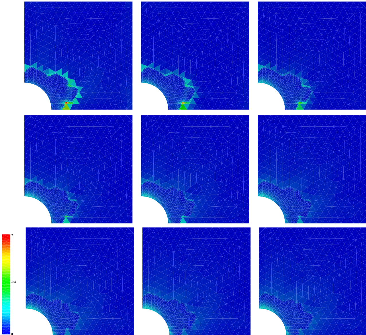
Figure 16: Scaled error map evolution: \theta_T(u_{Hh}^n)
