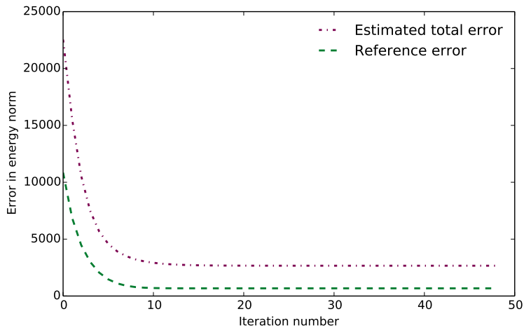
Figure 15: Evolution of the estimated total error \Theta(u_{Hh}^n) + \Theta_n and the reference error \Theta^{ref}
