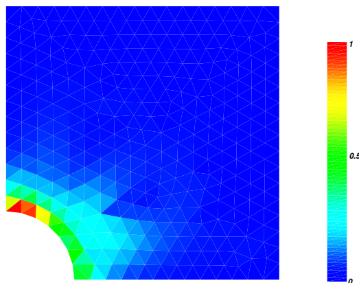
Figure 4: Relative residual error on the initial mesh
