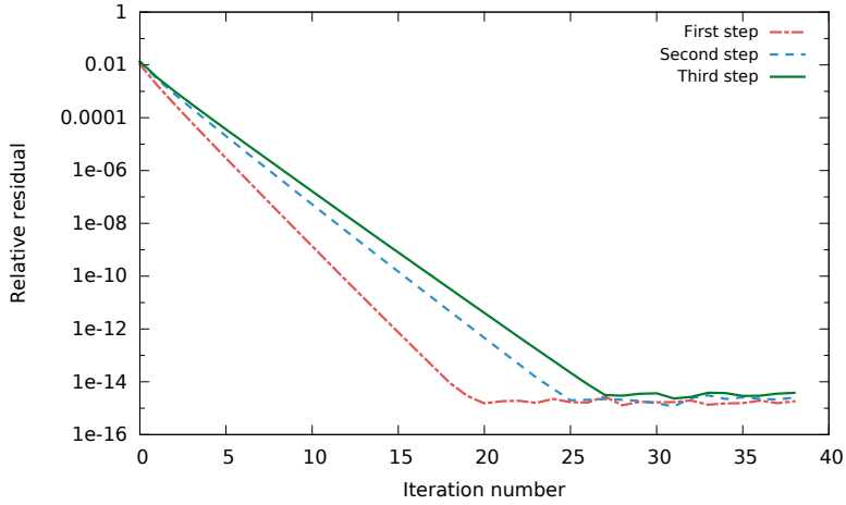
Figure 9: Evolution of the residual for each step of mesh refinement
