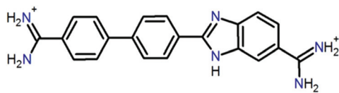
Fig. 1 Chemical structure of the heterocyclic cationic DB921.
