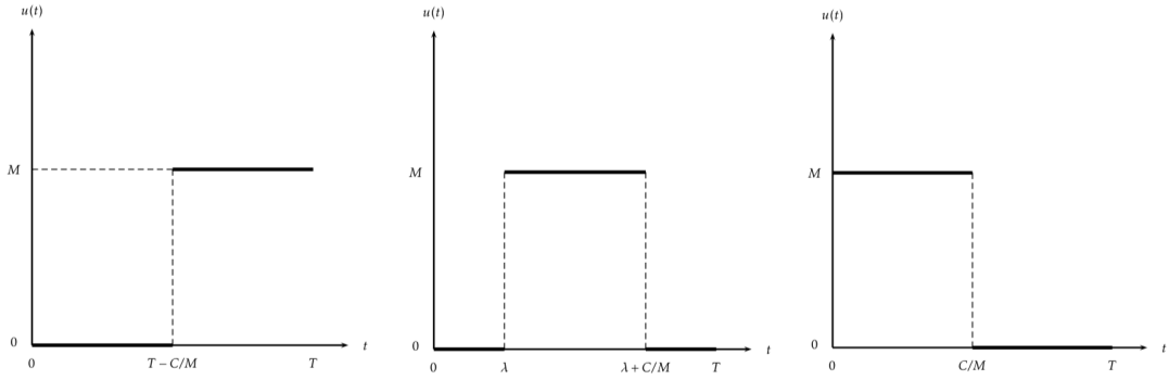
Figure 3: Left: solution u^* in the case M > \max_{p \in [0, \theta]} -f(p)/g(p) and C > C^*(M) . Middle: one solution u_\lambda^* in the case M > \max_{p \in [0, \theta]} -f(p)/g(p) and C = C^*(M) . Right: solution u^* in the case M \leq \max_{p \in [0, \theta]} -f(p)/g(p) or M > \max_{p \in [0, \theta]} -f(p)/g(p) and C < C^*(M) .
