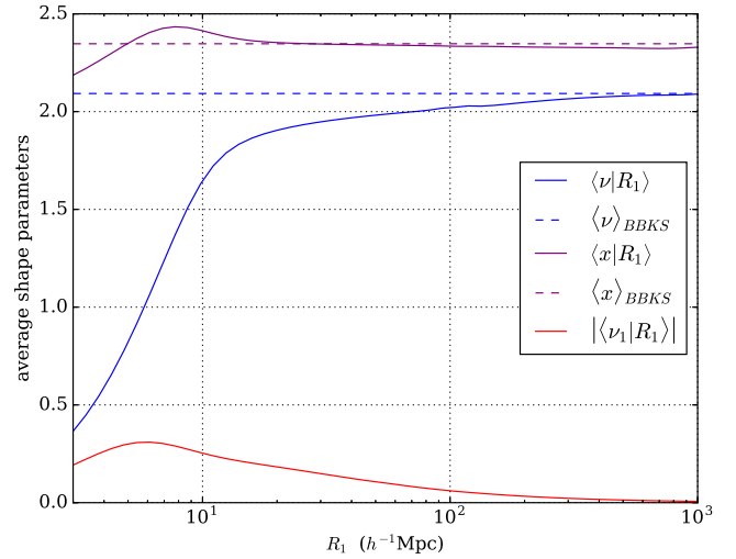
Figure 4. Mean expected values \langle X | R_1 \rangle for the shape parameters X = \{\nu, x, \nu_1\} computed from equations (50), (53), and (55) as a function of the compensation radius. For illustration, the \Lambda CDM matter power spectrum has been smoothed on a Gaussian scale R_f = 10 h^{-1} \text{Mpc} . The dashed lines are the expected values from BBKS with the condition equation (42) and are recovered for R_1 \rightarrow \infty as shown in Section 3.2.3. Note that \langle \nu_1 | R_1 \rangle \rightarrow 0 in the R_1 \rightarrow \infty limit.
