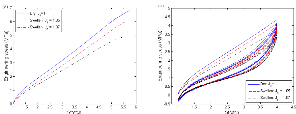
Figure 2. Result of the mechanical testing for (a) Test 1 (b) Test 2
