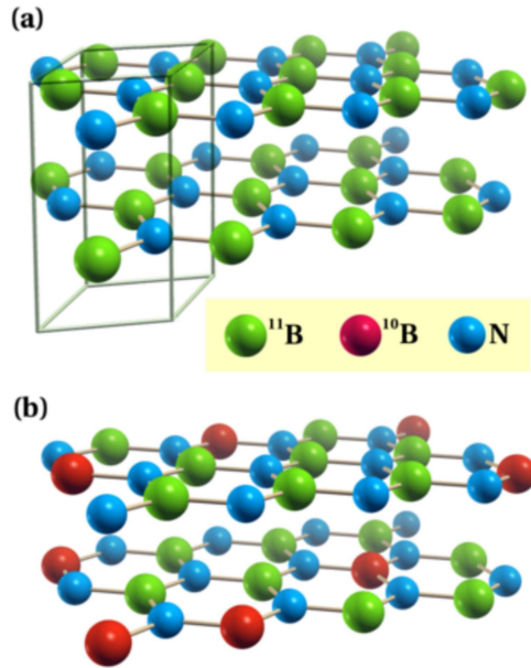
FIG. 1. Perspective view of a honeycomb bilayer conforming the crystalline structure of h -BN. The crystalline structure of h -BN consists of layers of flat, covalently bonded \text{B}_3\text{N}_3 hexagons anchored together by weak van der Waals forces. (a) Isotopically pure crystal. The primitive cell of the h -BN Bravais lattice containing two formula units is shown. (b) Natural isotopic composition (80% ^{11}\text{B} / 20% ^{10}\text{B} ) crystal with a random distribution of ^{10}\text{B} atoms at the cation sites.
