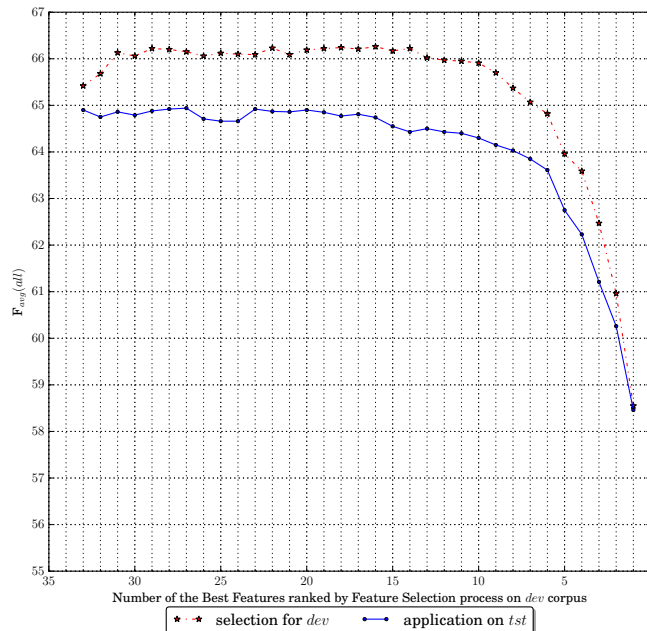
Figure 3 – Evolution of WCE performance for dev (features selected) and tst corpora when feature selection using SBS algorithm is made on dev ( ASR1 system only; the same shape is observed for ASR2 ).
