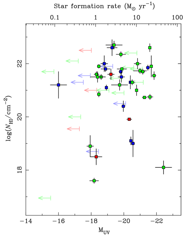
Figure 3. The values of neutral hydrogen column density plotted against host rest-frame UV absolute AB magnitude and corresponding star formation rate (top axis, following the calibration for a Z = Z_{\odot}/3 , constant star-formation rate and age > 300 Myr population from Madau & Dickinson 2014), for 37 detections and 19 upper limits collected from various sources (Table 1). Colour coding is as with the lines in Fig. 2 and upper limits are 2\sigma .
