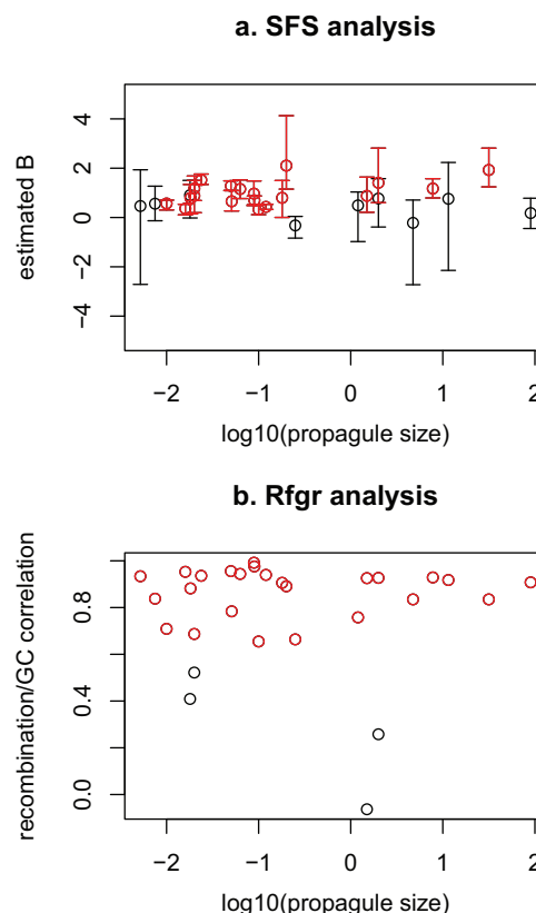
FIG. 5. Evidence for GC-biased gene conversion. Each dot represents a species. Top: SFS analysis; X axis: propagule size (log scale); Y axis: estimated scaled gBGC coefficient B ; red/darker dots: significant, positive B ; other dots: B not significantly different from zero. Error bars reflect 95% confidence intervals obtained by bootstrapping SNPs; Bottom: GC/recombination relationship; X axis: propagule size (log scale); Y axis: correlation coefficient between bins of R_{fgr} and bins of GC; red/darker dots: significant, positive correlation coefficient; other dots: correlation coefficient not significantly different from zero.
