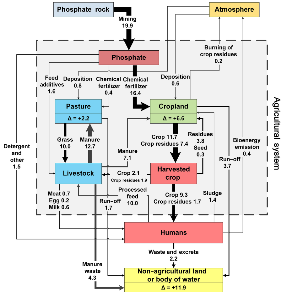
Figure 2. Annual P flows in the global agriculture system from 2002 to 2010. Values are Tg P yr -1 . The notation \Delta denotes the average change of P in pasture and cropland soils, respectively. By convention, a positive value means accumulation. Note that livestock and human changes of P are assumed to be zero.
