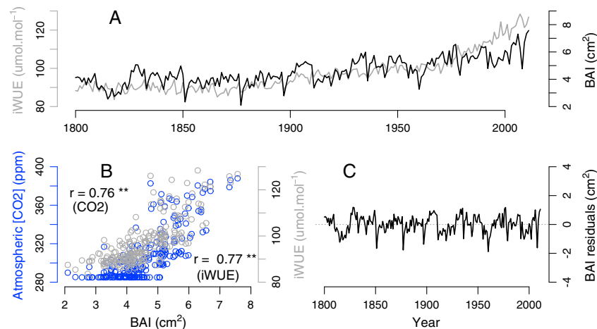
Figure 2. (a) Variations in intrinsic water-use efficiency (iWUE, gray) and basal area increment (BAI, black) over the 1800–2011 period. (b) Correlations between iWUE and atmospheric \text{CO}_2 (ppm) and BAI ( \text{cm}^2 ) over the same period. (c) Temporal variations of BAI residuals estimated using three different corrections (extracting iWUE or c_a trends from BAI series, or using a 50% spline; gray, blue and black, respectively). The ** indicates that the correlation is significant at 99% confidence level.
