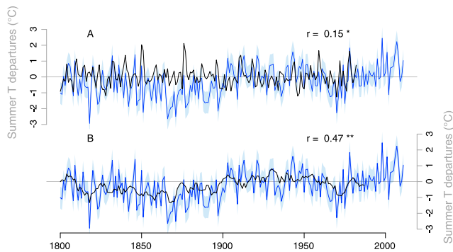
Figure 6. Comparison of the \delta^{13}\text{C}_{\text{cor}} -based (blue) reconstruction with (a) the Villalba (1990) summer reconstruction based on the treering width chronology of Fitzroya cupressoides at 41°S for the overlapping period 1800–1984 ( r = 0.15 , p < 0.05 ) and (2) the Villalba et al. (2003) reconstruction for the Northern Patagonian Andes based on the first principal component of tree ring width records from Nothofagus pumilio for the overlapping period 1800–1987 ( r = 0.47 , p < 0.01 ). The summer temperature anomalies are calculated using the 1901–1995 climatology. The shaded blue represents the confidence intervals for each reconstruction ( \pm 1 RMSE = 0.69^\circ\text{C} ). The * and ** indicate that the correlation is significant at 95% and 99% confidence level, respectively.
