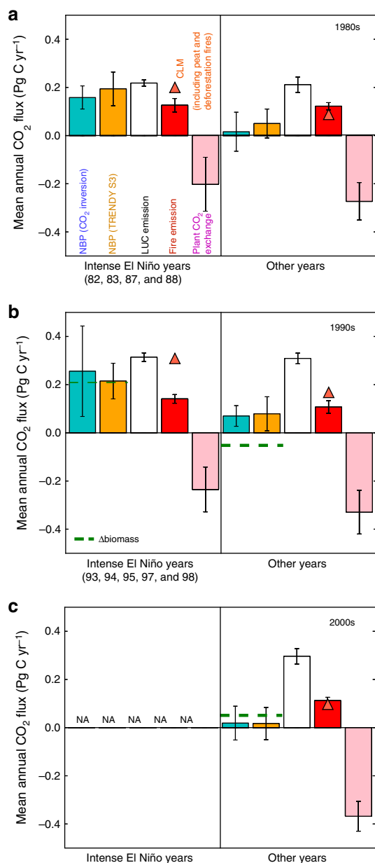
Fig. 4 Influence of the intense El Niño years on annual \text{CO}_2 fluxes of the past three decades. Comparison of mean annual \text{CO}_2 fluxes (NBP, LUC emissions, fire emissions and plant \text{CO}_2 exchange) between the intense El Niño years and rest of years for a the 1980s, b the 1990s and c the 2000s. Mean annual NBP from the atmospheric \text{CO}_2 inversions (cyan) and TRENDY S3 (orange) are shown for the three decades, and \Delta biomass (dashed green horizontal line) for the 1990s (1994–1999) and the 2000s (2000–2009). Component fluxes such as LUC emissions (white) and fire emissions (red), and plant \text{CO}_2 exchange (pink) are the estimates from the TRENDY S3. Fire emissions considering the attribution from peat and deforestation fires (the CLM model; orange triangles) are shown separately from an ensemble average of fire emissions by the other models. Error bars of each flux represent 1\sigma variation among models
