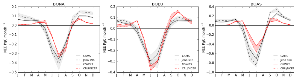
Figure 19. Monthly mean seasonal net land–atmosphere CO 2 fluxes (NEE in PgC month -1 ) from the GSWP3 and CRUNCEP-forced simulations compared to atmospheric inversions, over the three high-latitude sub-regions (shown in Fig. 2a), averaged over the period 2000–2007. The grey shaded areas correspond to the SD of the monthly values for each inversion. Note that a negative sign in NEE corresponds to CO 2 uptake from the atmosphere, and a positive sign to release into the atmosphere.
