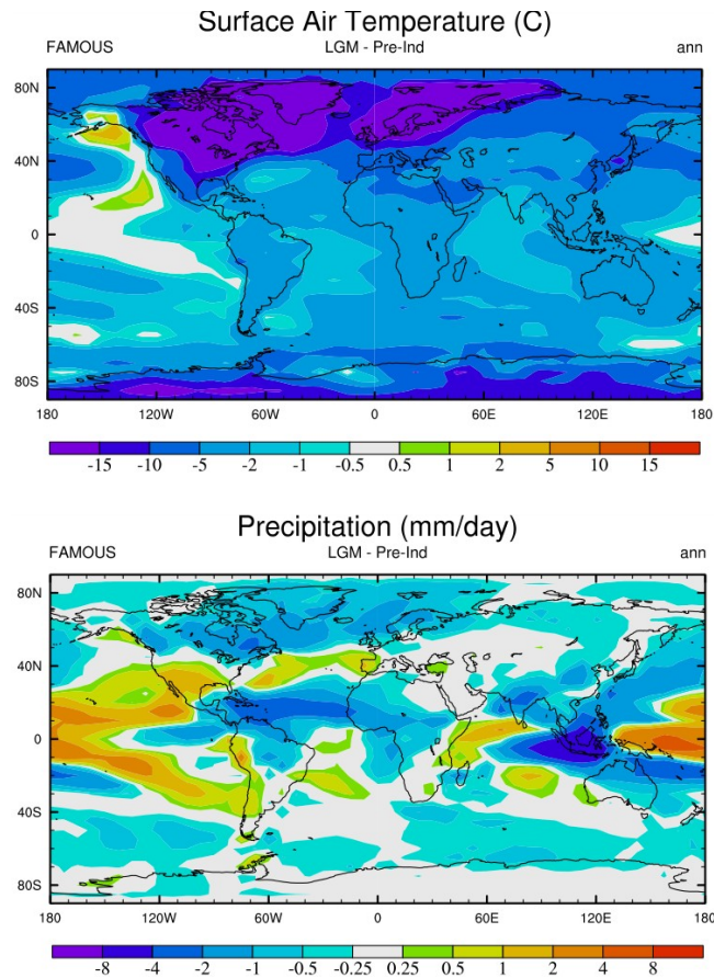
Fig. A1. LGM climate fields simulated by FAMOUS: surface temperature ( ^{\circ}\text{C} , top panel) and precipitation ( \text{mm day}^{-1} , bottom panel).
