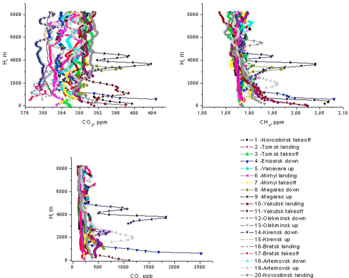
Figure 5. Vertical profiles of the CO 2 , CH 4 , and CO concentrations obtained in the flights of the 2012 campaign (averaged by smoothing in steps of 100 m on height).
