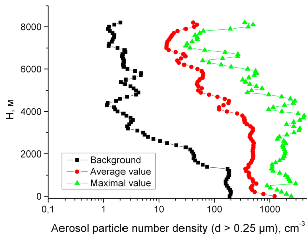
Figure 8. Background, average, and maximal number densities at the route (log scale).
