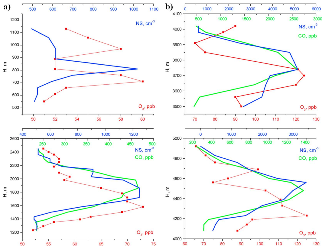
Figure 11. Vertical distribution of ozone (O 3 ), carbon monoxide (CO), and aerosol number density (NS) over Yakutsk (a) and Magaras (b).
