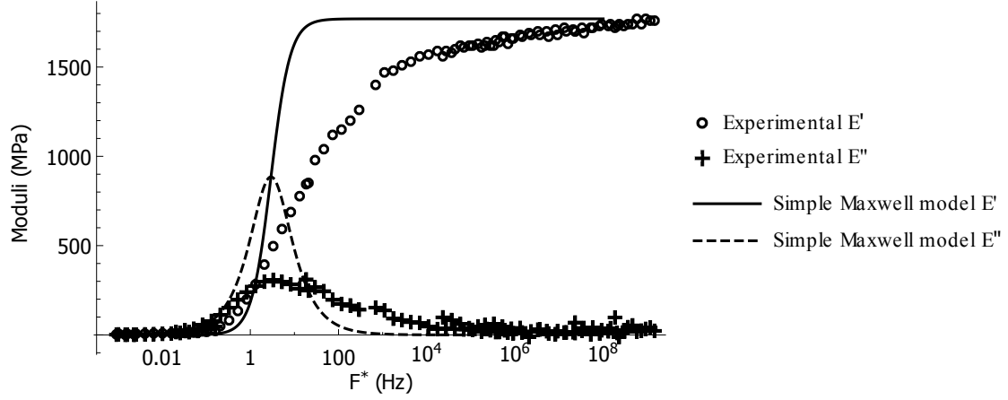
Fig. 4 Spring dashpot model fitted on the 150°C experimental master curve ( F^* = \frac{\omega^*}{2\pi} )
