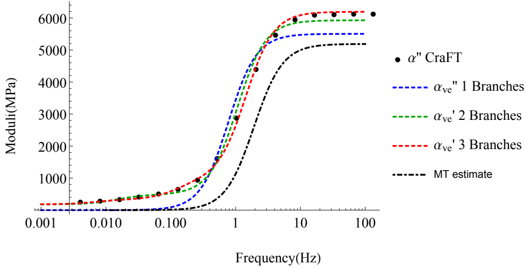
Fig. 18 Confrontation between storage moduli evolution identified with 1, 2 and 3 branches of spring dashpot models proposed, the reference values (numerical DMA with a full field method) and the classical MT estimate (numerical DMA with a mean field method)
