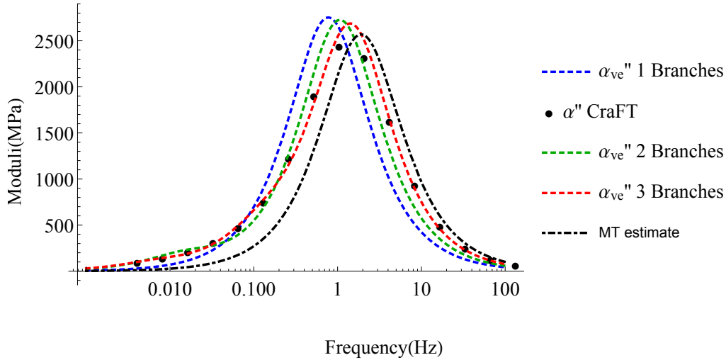
Fig. 19 Confrontation between loss moduli evolution identified with 1, 2 and 3 branches of spring dashpot models proposed, the reference values (numerical DMA with a full field method) and the classical MT estimate (numerical DMA with a mean field method)
