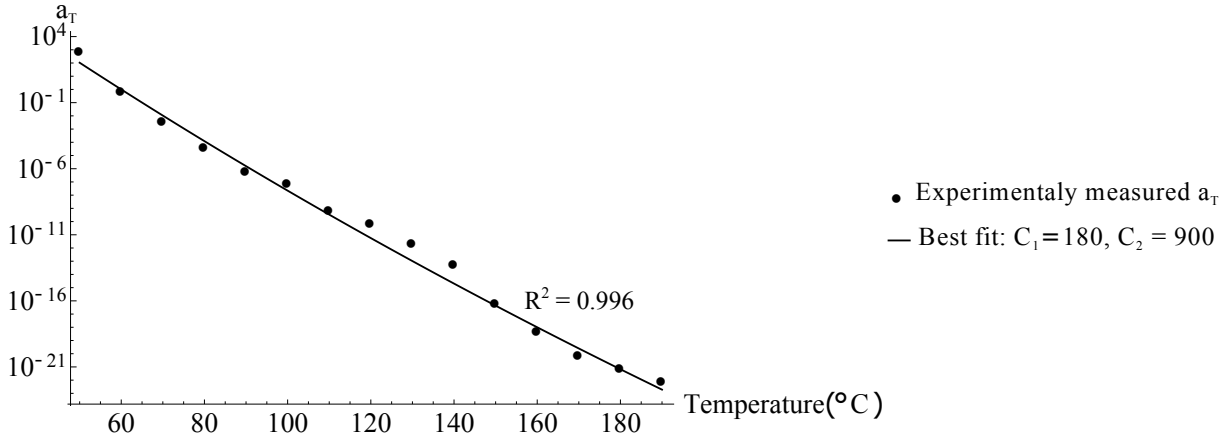
Fig. 3 Experimental value of a_T obtained with the TTS method and the corresponding best fit to identify the WLF law parameters ( C_1 and C_2 ), from 50°C to 190°C
