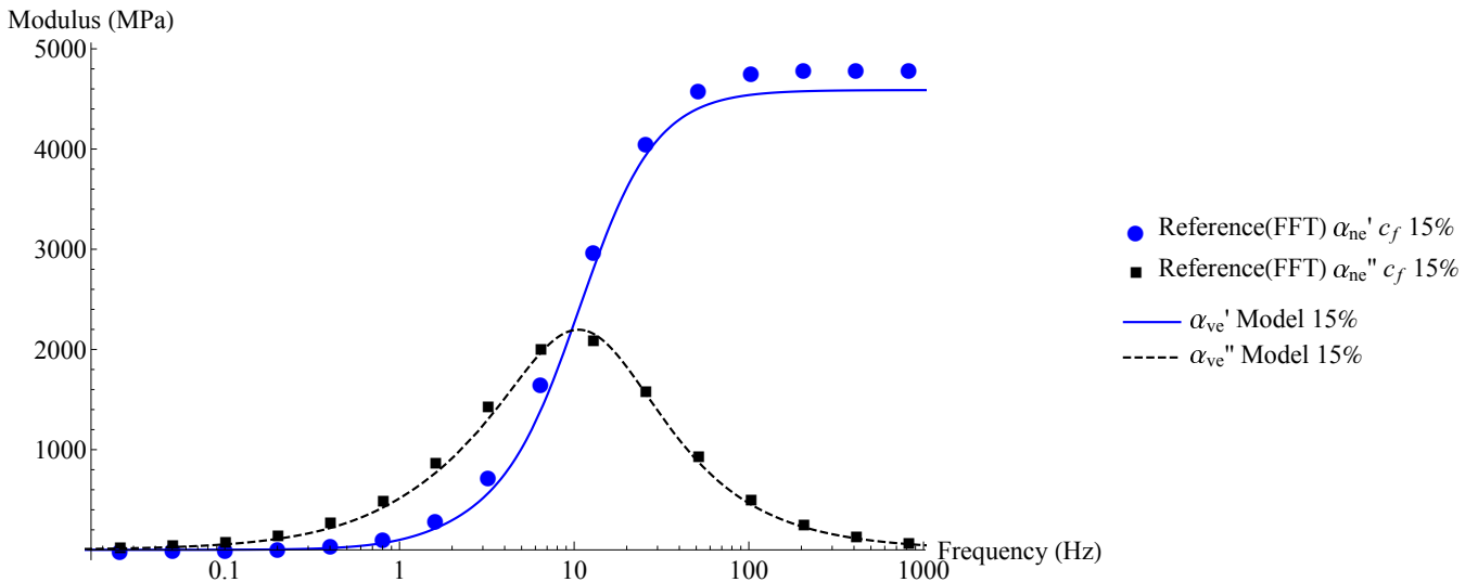
Fig. 25 comparison between the meta-model estimation and reference values obtained through FFT for 15% of fibers
