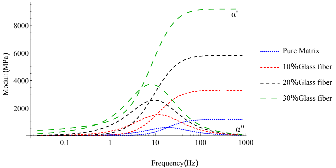
Fig. 16 Numerical DMA results: evolution of \alpha'_{ne} and \alpha''_{ne} moduli with fiber volume ratio change
