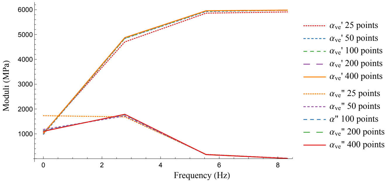
Fig. 9 Numerical DMA results on \alpha'_{ve} and \alpha''_{ve} moduli for five different number of time steps in one oscillation at four different frequencies
