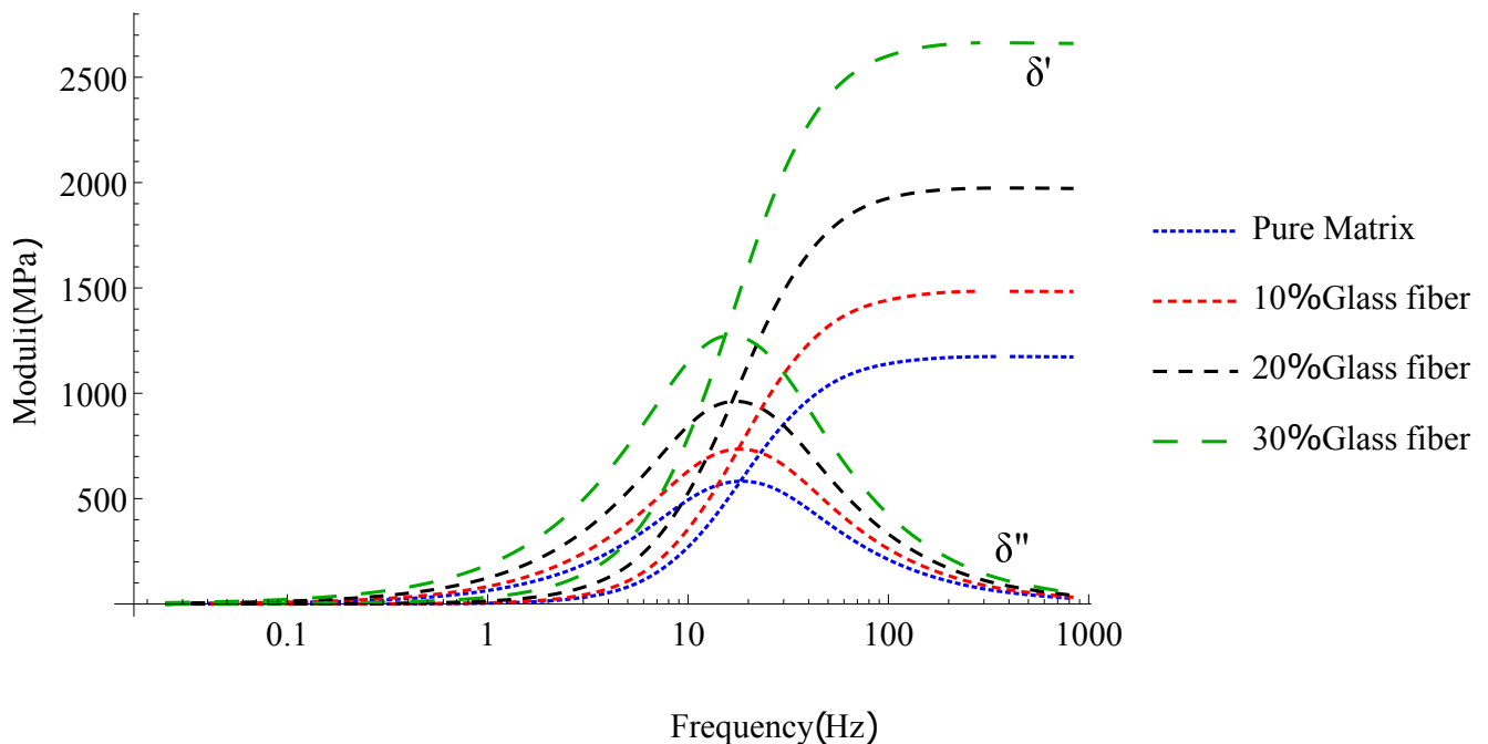
Fig. 17 Numerical DMA results: evolution of the \delta'_{ne} and \delta''_{ne} with fiber volume ratio change
