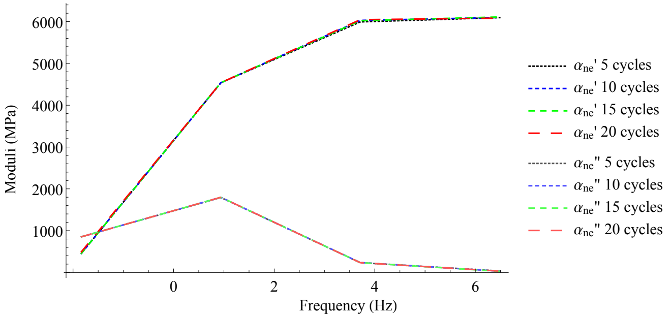
Fig. 8 Evolution of numerical DMA results on \alpha'_{ne} and \alpha''_{ne} moduli for four different numbers of cycle (only the 5 last cycles were processed each time to identify \alpha'_{ne} and \alpha''_{ne} ) at four different frequencies
