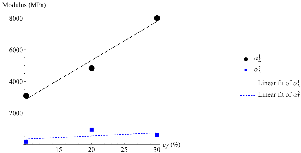
Fig. 22 Evolution of the \alpha_L parameters of the first two branches and best linear fit of it
