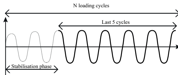
Fig. 7 Illustration of the convergence study on loading cycles, N cycles are processed, from 5 to 20, and in every cases the last 5 cycles are treated (to avoid the stabilisation phase)
