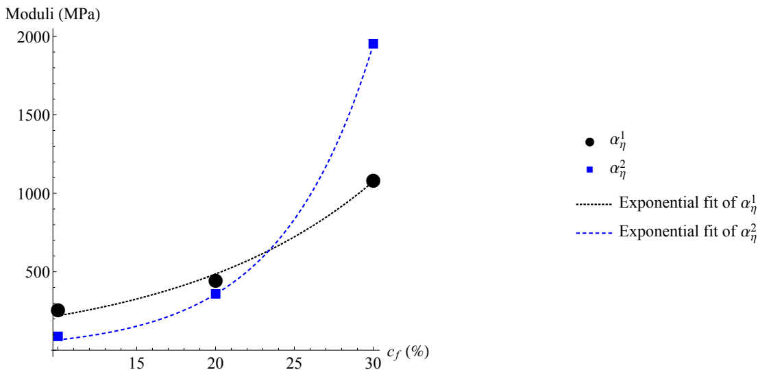
Fig. 23 Evolution of the \alpha_\eta parameters of the first two branches and its best exponential fit
