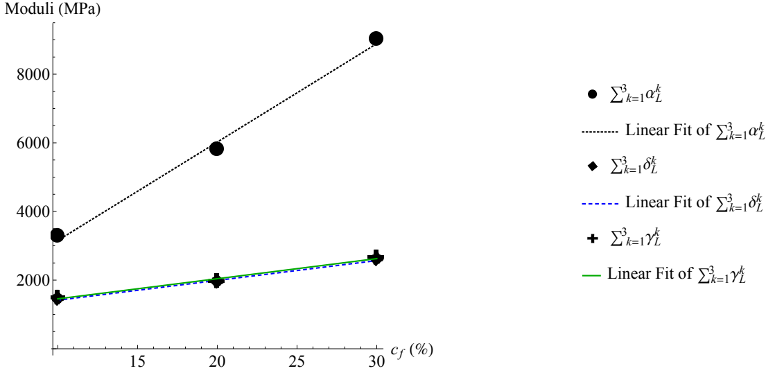
Fig. 20 Evolution of the sums of the elastic parameters with the fiber volume ratio variation, the best linear fit is also plotted.
