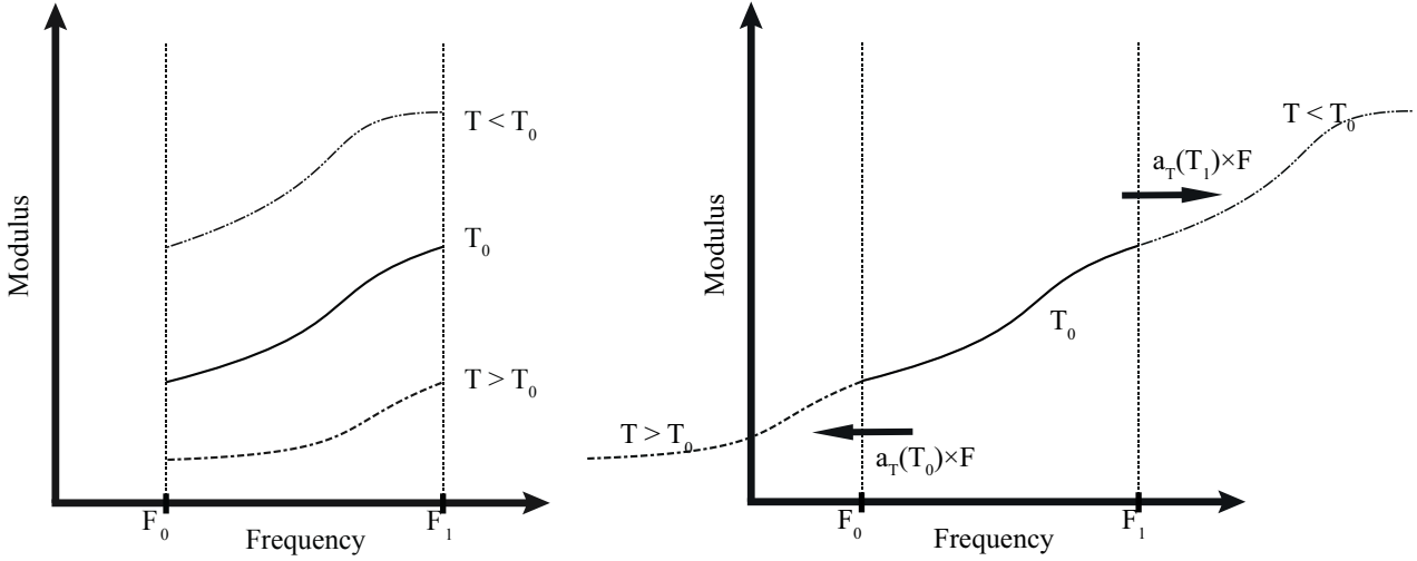
Fig. 2 TTS method illustrated, on the left are displayed the result of a temperature scan DMA, on the right are the a_T shifted results which then constitutes the master curve
