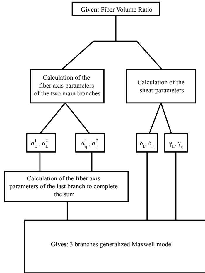
Fig. 24 Framework of the meta-model used to give the estimation of the behavior at a given fiber volume ratio
