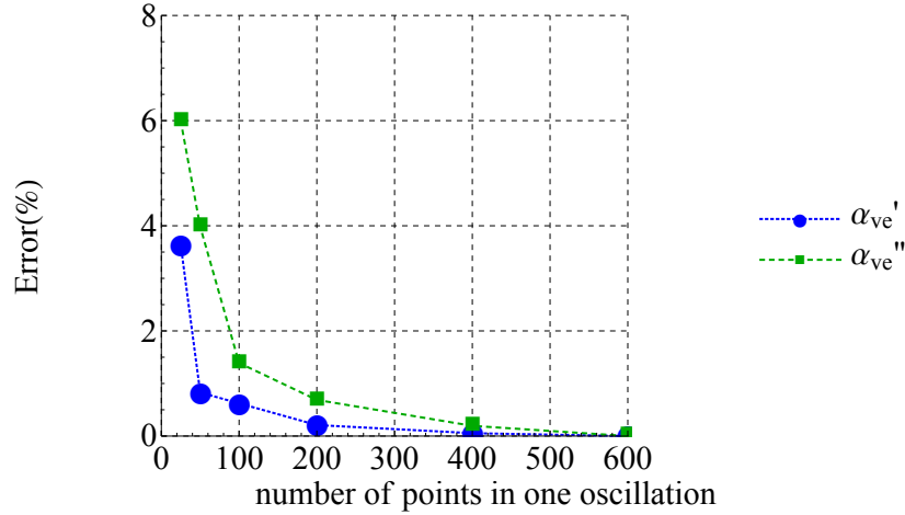
Fig. 10 Error on moduli calculation with our numerical DMA in function of DMA results sampling (considering the result for a sampling of 600 points as reference)
