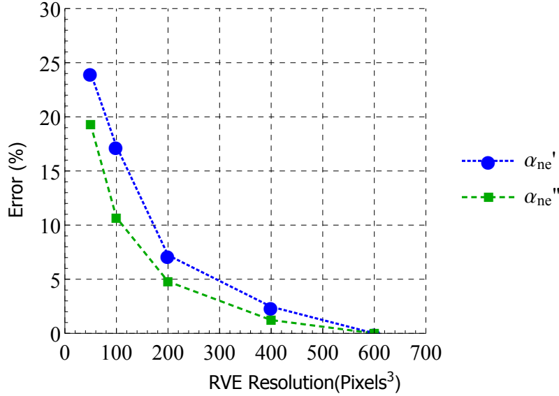
Fig. 12 Error on moduli calculation with our numerical DMA as a function of numerically generated RVE resolutions (considering the 600^3 pixels result as reference)
