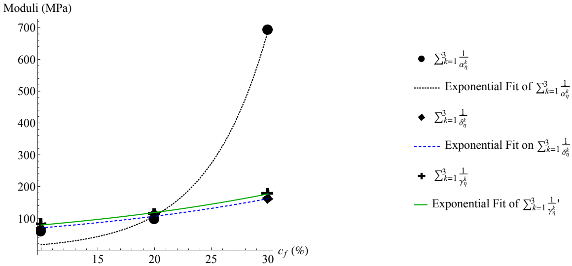
Fig. 21 Evolution of the inverse sums of the viscous parameters with the fiber volume ratio variation, the best exponential fit is also plotted.
