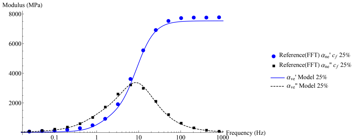
Fig. 26 Confrontation between the identified meta-model estimation and the reference values for 25% of fibers
