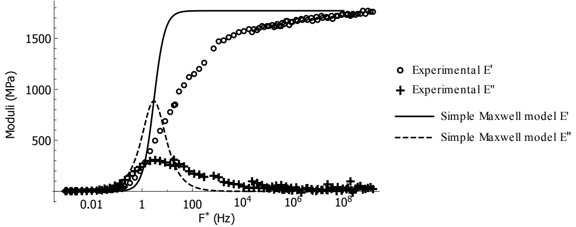
Fig. 4 Spring dashpot model fitted on the 150^{\circ}\text{C} experimental master curve ( F^* = \frac{\omega^*}{2\pi} )
