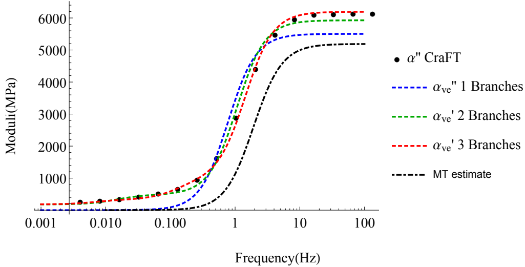
Fig. 18 Confrontation between storage moduli evolution identified with 1, 2 and 3 branches of spring dashpot models proposed, the reference values (numerical DMA with a full field method) and the classical MT estimate (numerical DMA with a mean field method)
