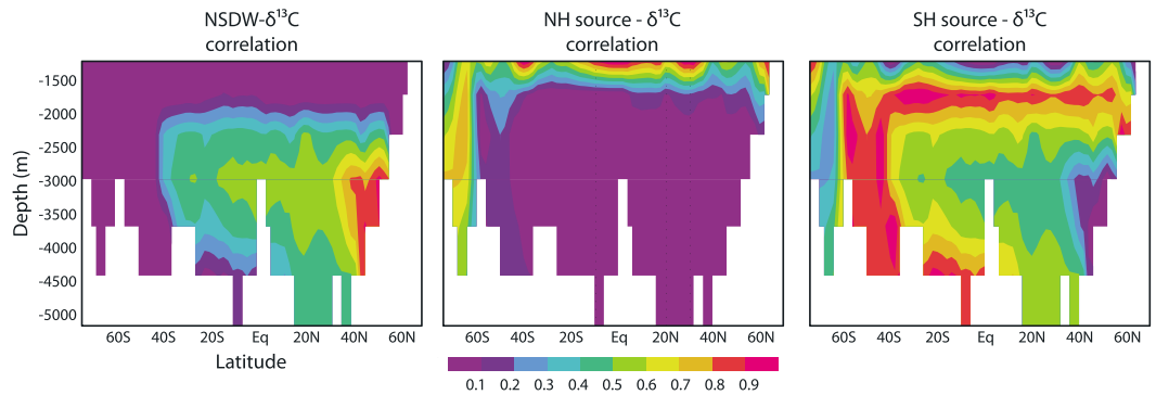
Figure 7. Meridional-depth cross section of correlation between NSDW, NH source, SH source, and \delta^{13}\text{C} . The cross section follows roughly the western boundary of the Atlantic basin (see Figure 1 for exact path) and is based on single grid cell values. See caption of Figure 6 for more information.
