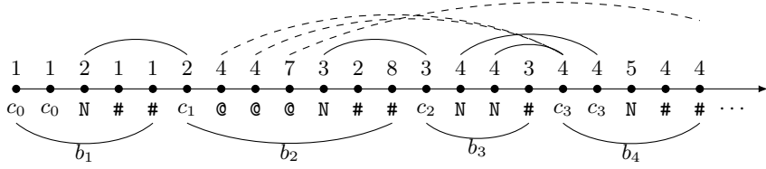
Fig. 2. \text{LTL}_1^\downarrow(\mathbb{F}) cannot avoid having repeated consecutive symbols.
