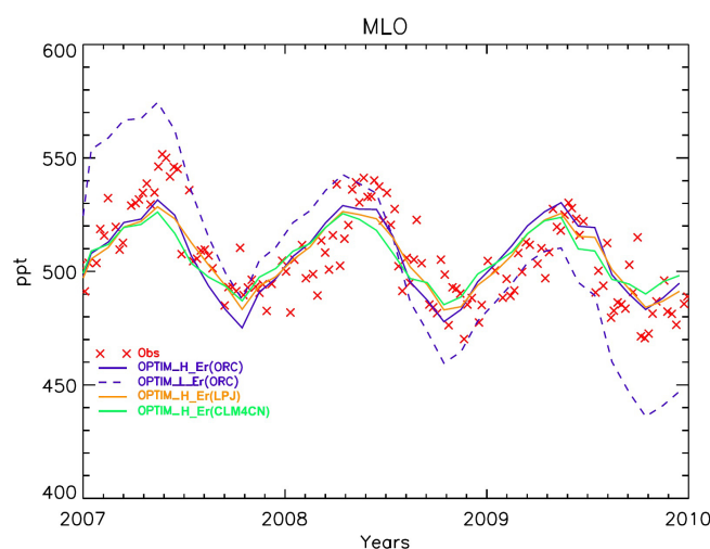
Figure 8. Annual variations of OCS monthly mean mixing ratios (in ppt), optimized and monitored at Mauna Loa. Simulations obtained with the LMDZ model using the OPTIM_H-Er setup (Table 1) applied to ORC, NCAR-CLM4 and LPJ models. Observations (red crosses) are from the NOAA/ESRL global monitoring network (Montzka et al., 2007). A sensitivity test was carried out using ORC and the OPTIM_L-Er setup (dashed blue line).
