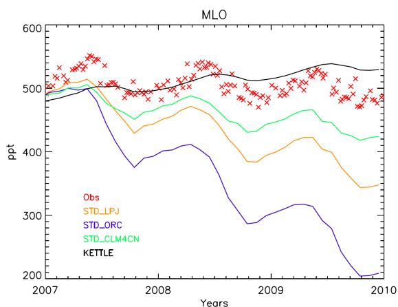
Figure 2. Annual variations of OCS monthly mean mixing ratios (in ppt), simulated and monitored at Mauna Loa. Simulations with the LMDZ model use the STD_ORC, STD_LPJ and STD_CLM4CN configurations described in Table 1. Data derived solely from the Kettle et al. (2002) surface fluxes are shown by the black solid line. Observations (red crosses) are from the NOAA/ESRL global monitoring network (Montzka et al., 2007).
