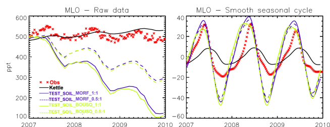
Figure 4. Sensitivity tests performed using the TEST_Soil_MORF_0.5:1, TEST_Soil_MORF_1:1, TEST_Soil_BOUSQ_0.5:1 and TEST_Soil_BOUSQ_1:1 setups of surface fluxes (Table 1) to simulate annual variations of OCS monthly mean mixing ratios (left panel) and smoothed seasonal variations obtained after removing the annual trends (right panel), at Mauna Loa. The simulations based solely on the Kettle et al. (2002) surface fluxes are shown by the black solid line. Observations (red crosses) are from the NOAA/ESRL global monitoring network (Montzka et al., 2007).
