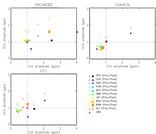
Figure 12. Scatter plots of normalized amplitudes of smoothed seasonal cycles of OCS versus those of CO 2 , before (open symbols) and after optimization (filled symbols) of OCS fluxes at 10 stations of the NOAA monitoring network, obtained from the STD_ORC, STD_CLM4CN and STD_LPJ setups for the forward simulations and the OPTIM_H-Er setup for the optimizations, over the period 2006–2010. Since the amplitude of the seasonal cycle in the observations at each site is used to normalize that of the simulations, the normalized amplitude of observations is 1 (red cross). Hence, a linear translation along the y axis towards Y = 1 characterizes the optimization process.
