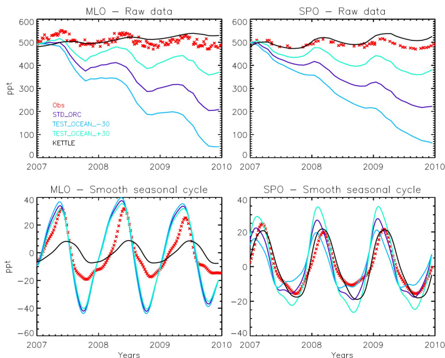
Figure 3. Sensitivity tests performed using the TEST_Ocean \pm 30 setup of surface fluxes (Table 1) to simulate the annual variations of OCS monthly mean mixing ratios (upper panels) simulated and monitored at Mauna Loa (left column) and South Pole (right column). Raw data were fitted with a function including a polynomial term (first order) and four harmonics. The residuals of the functions were further smoothed in the Fourier space, using a low-pass filter (cutoff frequency of 65 days) to define a so-called smoothed curve (function plus filtered residuals). The mean seasonal cycle is defined from the smoothed curve after subtraction of the polynomial term. The corresponding smoothed seasonal variations obtained are displayed in lower panels. The simulations based solely on the Kettle et al. (2002) surface fluxes are shown with a black solid line. Observations (red crosses) are from the NOAA/ESRL global monitoring network (Montzka et al., 2007).
