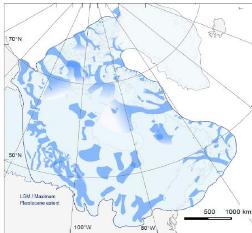
Figure 5: The number of hypothesised ice streams has grown rapidly over recent years, with those in the Laurentide Ice Sheet increasing from 10 (black arrows) that were reviewed by Stokes and Clark (2001) in (a), to over 100 (blue shading) in the latest inventory compiled by Margold et al. (2015) in (b).
