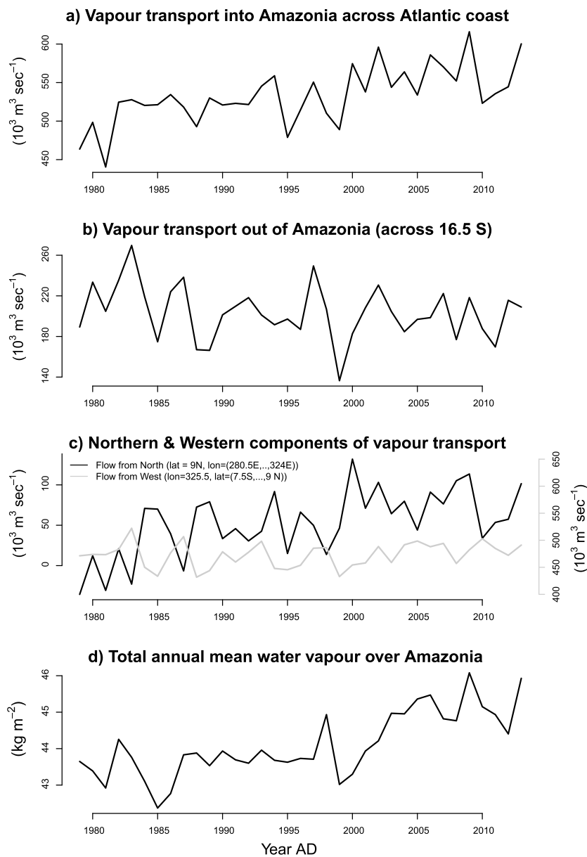
Figure 5. (a) Water vapor transport into Amazon basin (across line 2 in Figure 4), (b) water vapor outflow (across line 4 in Figure 4), (c) water vapor transports across lines 1 and 3 in Figure 4, and (d) water vapor content over the Amazon basin, all based on ERA-Interim reanalysis [Dee et al., 2011].
