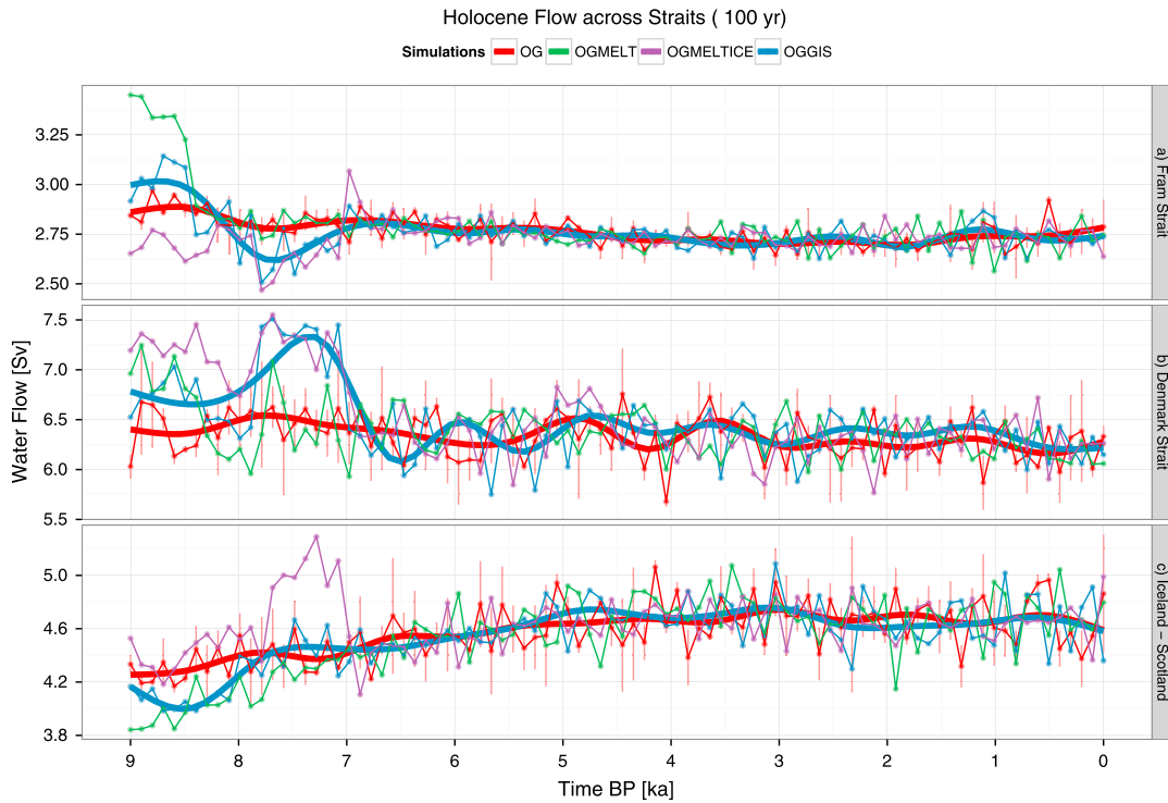
Figure 7. Modeled flow across the major pathways in the North Atlantic, the Fram Strait, the Denmark Strait, and the Iceland-Scotland Ridge. Shown are 100 year averages of bottom current strength in sverdrup for four simulations (OG, OGMELT, OGMELTICE, and OGGIS). Thick lines represent smoothed values ( n = 9 ), and red bars indicate the standard deviation of simulation OG.
