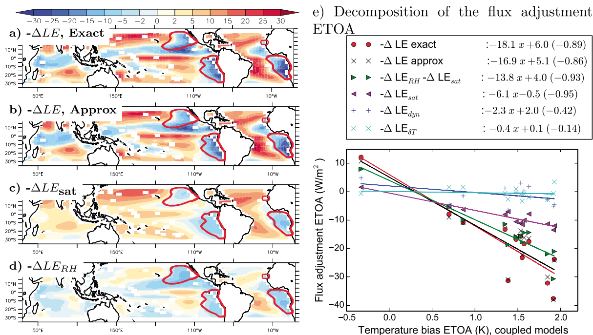
Figure 3. Decomposition of the latent heat flux adjustment \Delta LE (in W/m^2 ) between stand-alone and coupled atmospheric simulations. The latent heat flux adjustment is approximated as the sum of four contributions, respectively, due to changes in wind speed ( \Delta LE_{dyn} ), saturation humidity ( \Delta LE_{sat} ), relative humidity ( \Delta LE_{RH} ), and sea-air temperature contrast ( \Delta LE_{\delta T} ). (a–d) The geographical distribution of the actual and approximate flux adjustments, as well as the contributions of changes in saturation humidity and in relative humidity to this flux adjustment are shown, respectively. (e) The multimodel scatterplot of the actual and the approximate flux adjustment ETOA as well as the multimodel scatterplot of their various contributions are shown as a function of the surface temperature bias ETOA in the coupled simulations. For this figure, the same 13 models were retained as in Figure 1d.
