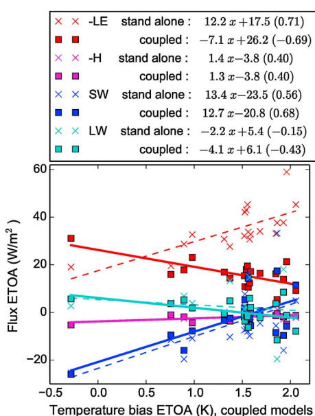
Figure 2. Adjustment between fluxes in atmosphere-alone simulations and temperature in coupled simulations. (a) Multimodel scatterplot of the atmospheric flux ETOA (in W/m^2 ) in stand-alone atmospheric (crosses and dashed regression lines) and ocean-atmosphere coupled (squares and full lines) simulations as a function of the temperature bias ETOA in coupled simulations. Fluxes are decomposed into latent ( -LE ) and sensible ( -H ) heat flux and short-wave (SW) and long-wave (LW) radiation. The results of ACCESS1-3 were ignored due to missing upward radiation in the historical simulation. (b) Sketch of the main processes involved in the control of air-sea fluxes, illustrating the control of SW and LW radiation by clouds as well as the various components of the water vapor transport controlling the near-surface humidity and the evaporation. (c) Summary of the atmospheric fluxes ETOA at the origin of the warm bias (stand-alone simulations; red arrows) and of the response of the surface fluxes to this temperature bias (difference between coupled and stand-alone simulations; blue arrows). The numerical values are deduced from the slopes of the regression lines of Figure 2a and are given in W/m^2 for a 1 K SST ETOA bias.
