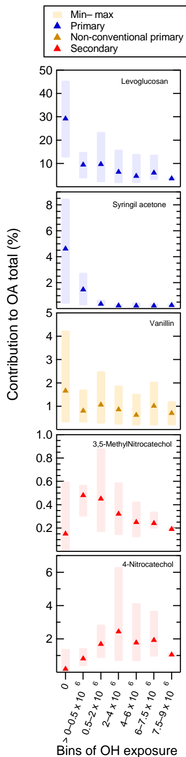
Figure 8. Evolution of the contribution of several markers to the OA(t) mass concentration at different time points in the photo-oxidation process. The marker represents the mean value over all experiments within a specific range of integrated OH exposure. The box includes the minimum and maximum within the same range.
