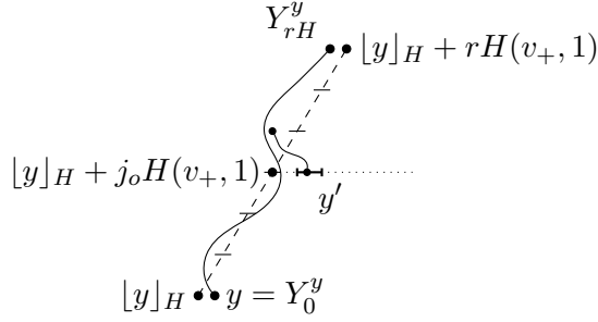
Figure 3: The point [y]_H is (H, r) -threatened, since [y]_H + j_o H(v_+, 1) is H -trapped.
