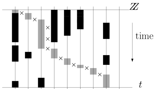
Figure 5: [Blo13] In grey, a trajectory of a distinguished zero up to time t ; time goes downwards, sites are highlighted in black at the times when they are occupied. The crosses represent clock rings at the site occupied by the distinguished zero.
