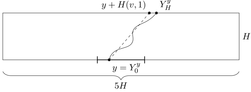
Figure 1: An illustration of the event A_{H,o}(v) . Starting from the point y \in ([0, H) \times \{0\}) \cap \mathbb{L} the walker attains an average speed larger than v during the time interval [0, H] .
