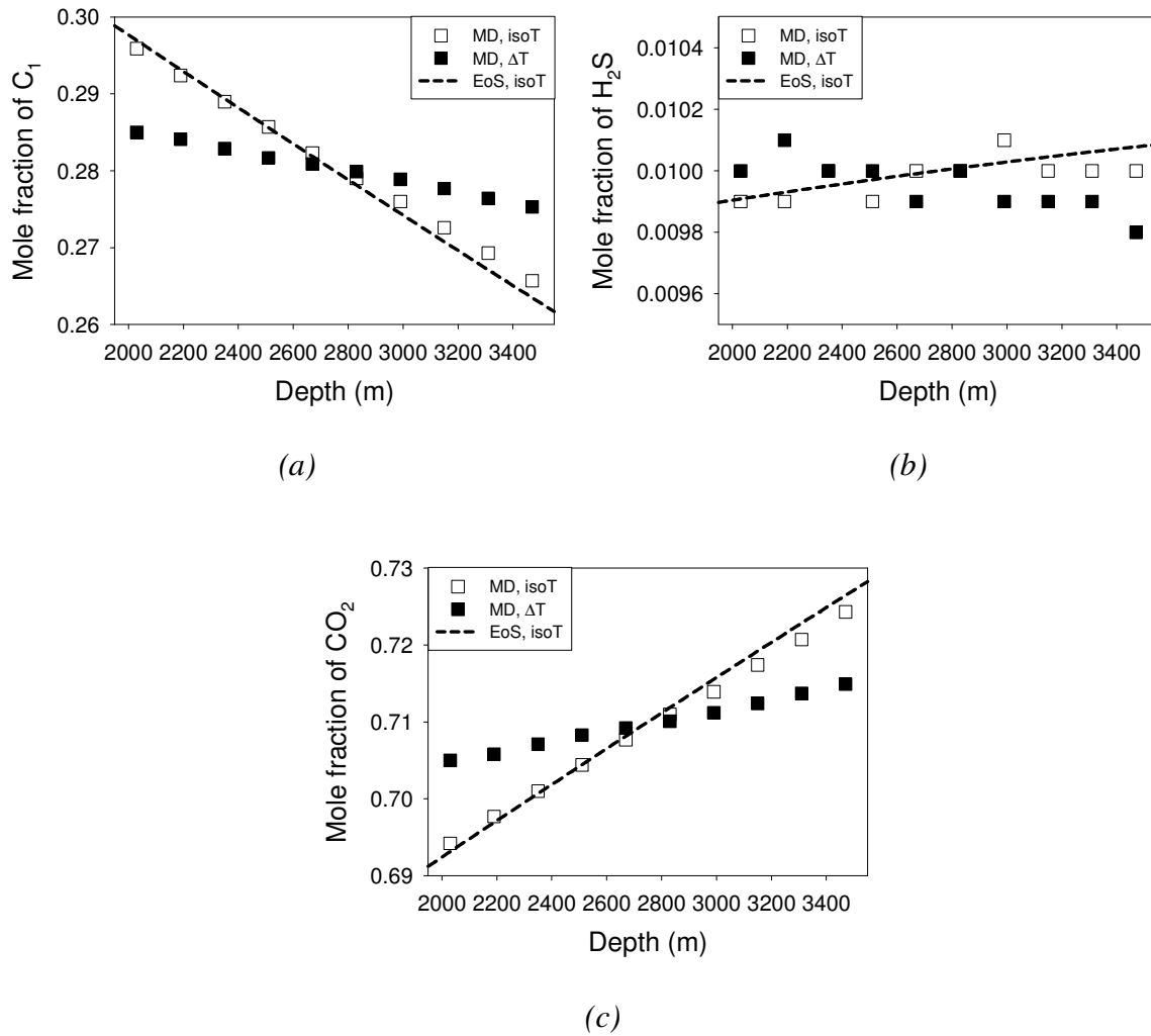
Figure 4: Mole fractions versus depth in a ternary CO_2 - C_1 - H_2S mixture subject to segregation ( isoT ) and thermogravitation ( \Delta T ) using MD simulations and thermodynamic modelling.
