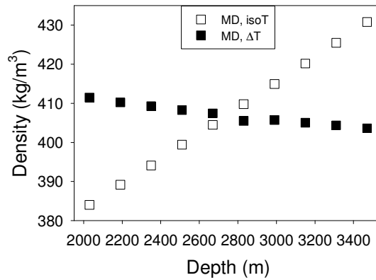
Figure 5: Densities versus depth in an acid gas mixture subject to segregation ( isoT ) and thermogravitation ( \Delta T ).
