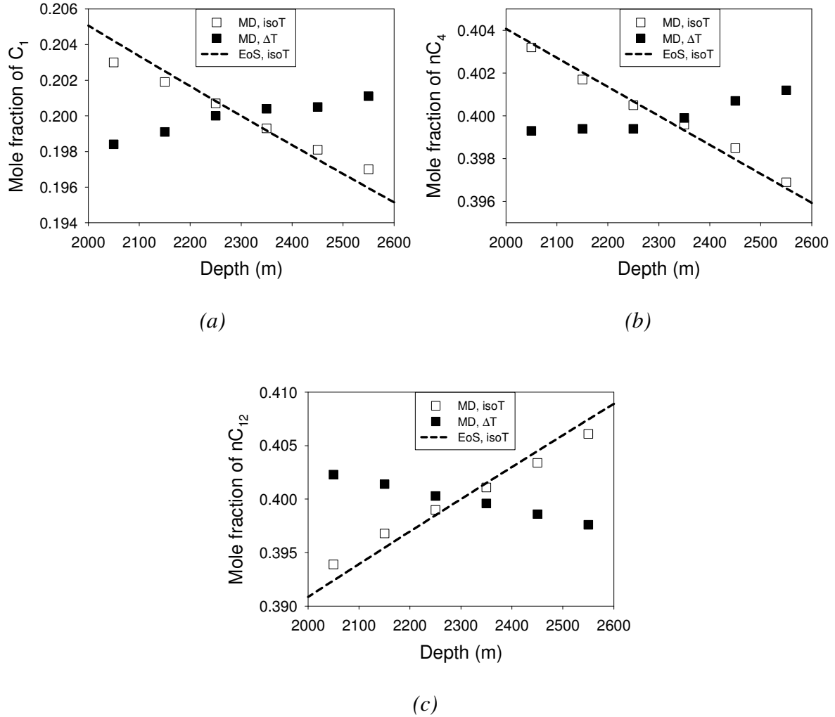
Figure 2: Mole fractions versus depth in a ternary C_1 - nC_4 - nC_{12} mixture subject to segregation ( isoT ) and thermogravitation ( \Delta T ) using MD simulations and classical thermodynamic modelling.
