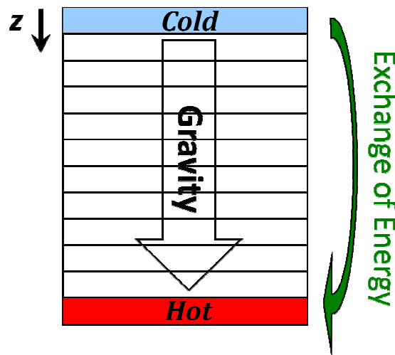
Figure 1: A sketch of the scheme employed to study thermogravitation using MD simulations (only half of the simulation box is shown).
