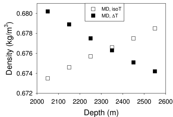
Figure 3: Densities versus depth in a ternary C_1 - nC_4 - nC_{12} mixture subject to segregation ( isoT ) and thermogravitation ( \Delta T ).
