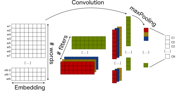
Figure 1: CNN for Text Classification
