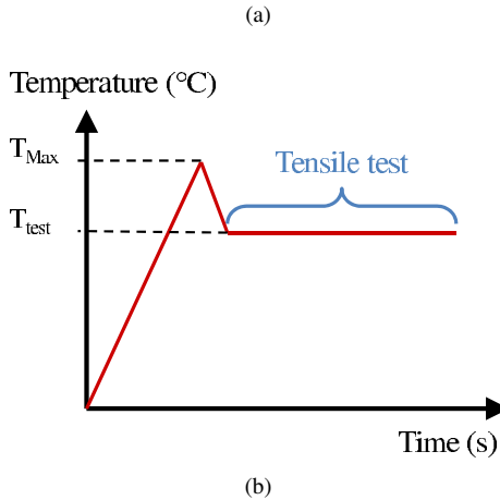
Figure 1: Tensile test procedure from T6 state: (a) after heating and (b) after overheating and partial cooling.
