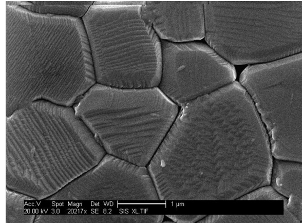
Fig. 12 – SEM images showing grain boundaries of \gamma\text{-Al}_2\text{O}_3 samples sintered at 1700\ ^\circ\text{C} with 5\ ^\circ\text{C}/\text{min} heating rate.
