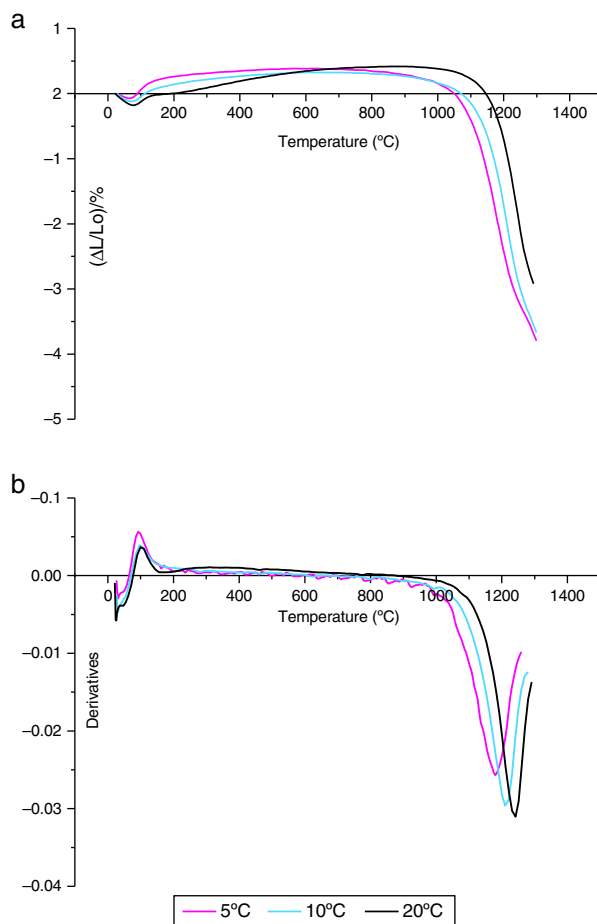
Fig. 5 – Dilatometry curves (a) and their derivatives (b) of the \gamma -Al 2 O 3 transition alumina samples heated up to 1300 °C for different heating rates.
