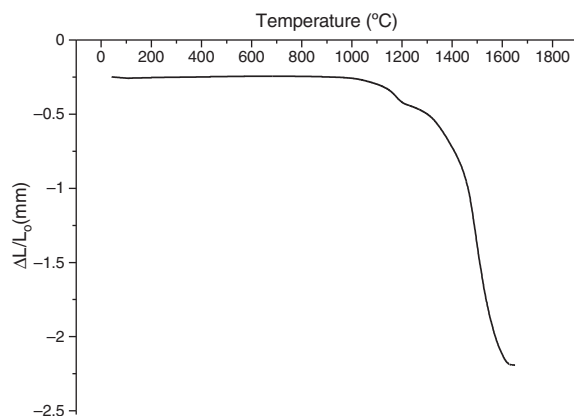
Fig. 6 – Dilatometry curve of the \gamma -Al 2 O 3 transition alumina sample heated up to 1700 °C at 5 °C/min heating rate.
