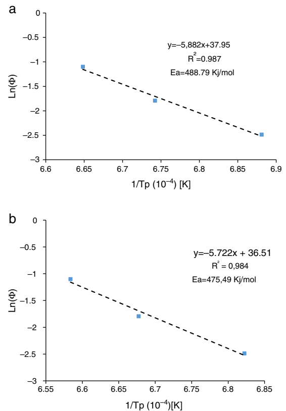
Fig. 10 – Plots of \ln\Phi versus 1/T_p (a) by dilatometry curves, (b) by DTA curves.
