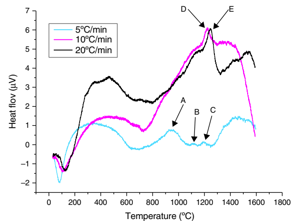
Fig. 4 - DTA curves of the \gamma\text{-Al}_2\text{O}_3 raw powder up to 1600^\circ\text{C} for different heating rates.
