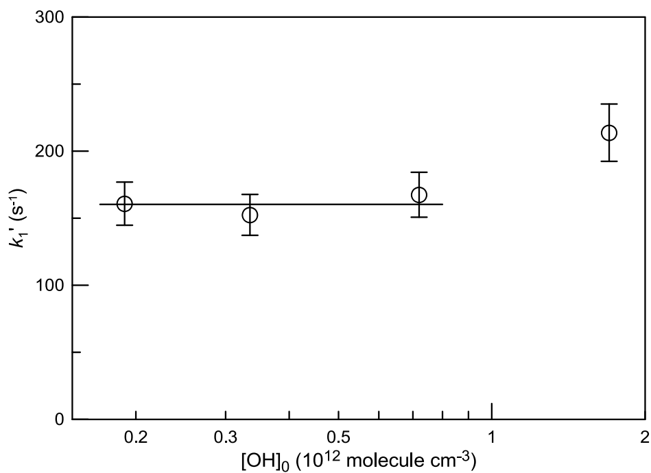
Fig. S4. Reaction \text{OH} + 2\text{-methyl-1-butyl nitrate} , T = 298 K, [2\text{M1BNT}] = 6.5 \times 10^{13} \text{ molecule cm}^{-3} : dependence of k_1' on initial concentration of OH radicals.
