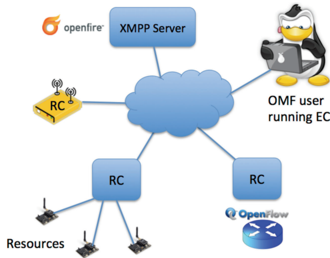
Figure 12.3 OMF 6 architecture.
