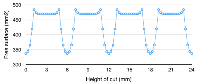
Fig. 5. Free surface function of the height of cut.
