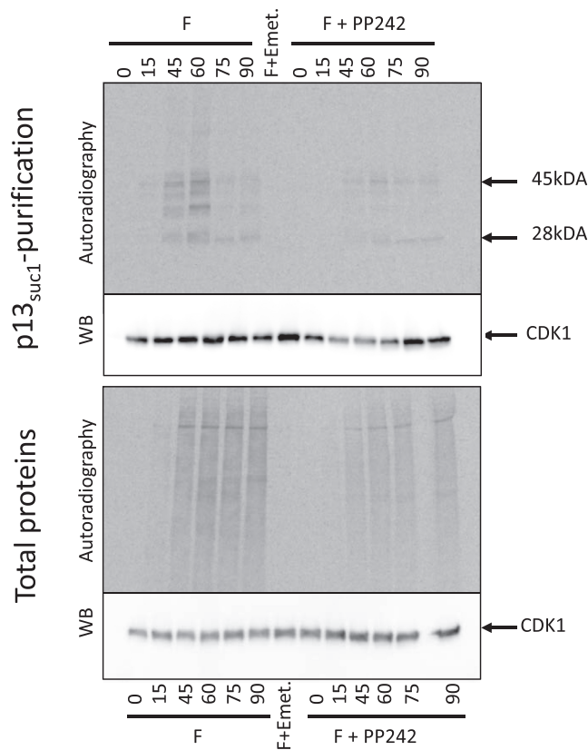
Figure 5. CDK1 protein is newly synthesized after fertilization. [ ^{35}\text{S} ]-methionine labeled proteins from embryos collected at the indicated times after fertilization were incubated on p13 suc1 -sepharose beads; affinity-purified proteins were resolved on SDS-PAGE and transferred to a nitrocellulose membrane. After exposure on a PhosphorImager screen (autoradiography), the membrane was incubated with anti-PSTAIR antibodies directed against the CDK1 protein (WB). Autoradiography and western blot on total proteins are shown in the bottom panel. Fertilized (left) and PP242-treated (right) embryos are shown. As a control, [ ^{35}\text{S} ]-methionine labeled embryos were cultured in presence of emetine, which was added 5 min after fertilization to inhibit protein synthesis, and the lysate prepared from embryos harvested at 90 min was used for p13 suc1 -sepharose bead purification (F+emetet). The experiment was performed twice.
