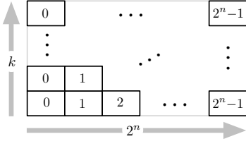
Fig. 4. 2^n corridor tiling. Each depicted box contains a tile from T . Each number inside a box is the index of the position.
