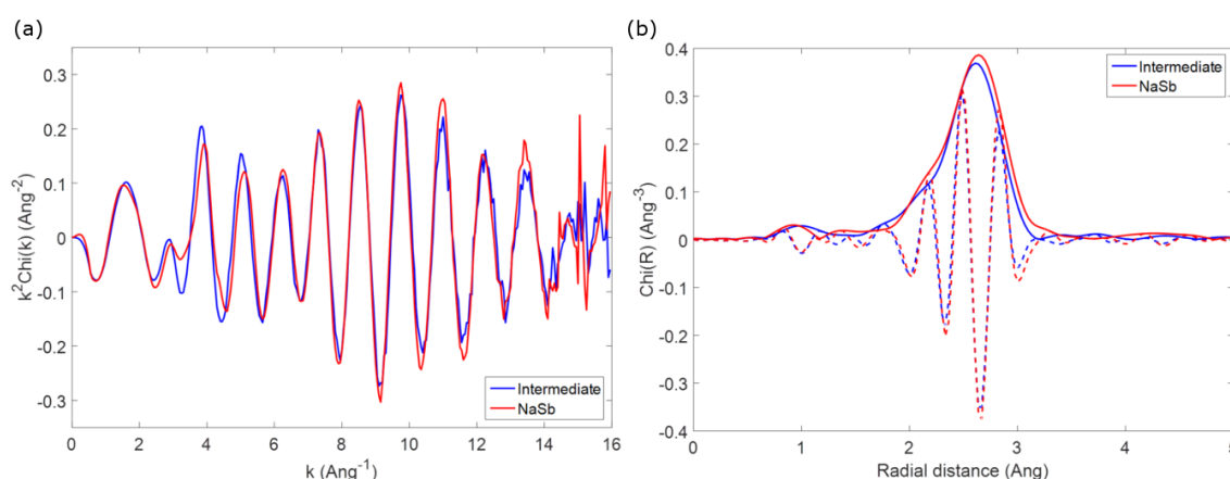
Figure 5. EXAFS spectra (a) and respective Fourier Transform (b) of NaSb (red) and of the Sb electrode after the reaction of about 1 mol Na per mol of Sb during the second discharge (blue).
