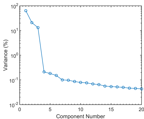
Figure 3. Variance plot obtained by the Principal Component Analysis of EXAFS operando spectra. Three components containing almost 98% of total spectra information stand out, the residuals represent the experimental noise.
