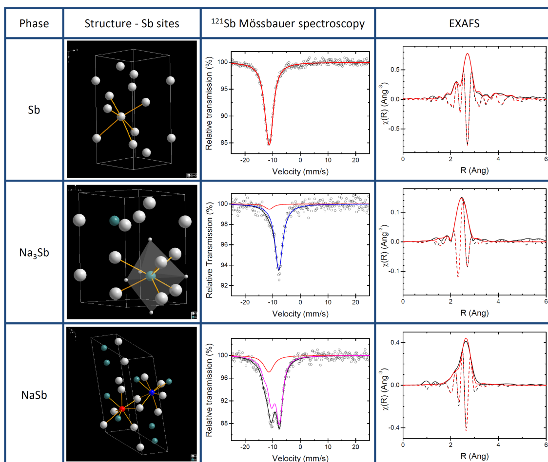
Figure 1. From (left) to (right): Local coordination of the Sb centres, 121 Sb Mössbauer and EXAFS spectra of reference compounds Sb, Na 3 Sb (Sb atoms in green) and NaSb (red and blue atoms identify the two Sb sites).
