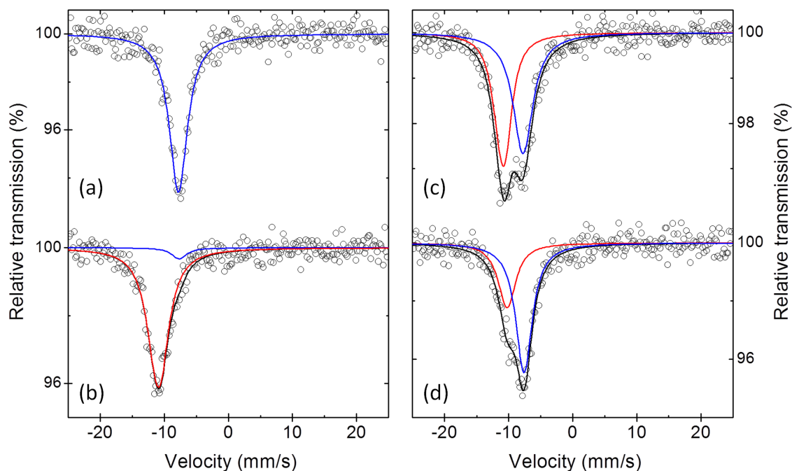
Figure 6. 121 Sb Mössbauer spectra at 78 K of Sb electrodes at the end of first discharge (a), at the end of first charge (b), after the reaction of 1.5 mol Na during first discharge (c) and after reaction of 2 mol Na during the first discharge (d).
