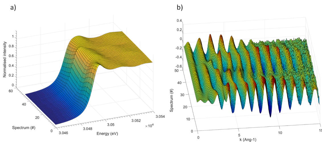
Figure 2. XANES (a) and EXAFS (b) operando Sb K-edge spectra measured during the first one and a half electrochemical cycles of Sb electrode vs. Na.
