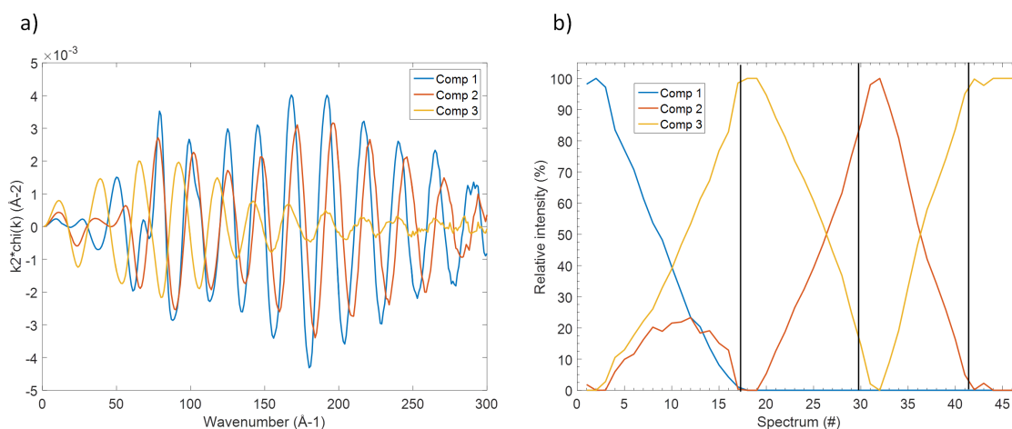
Figure 4. EXAFS spectral components (a) obtained by MCR-ALS analysis of the EXAFS operando spectra, and variation of their intensity (b) during electrochemical cycling. The vertical black lines represent the end of each process (first discharge, first charge, and second discharge).
