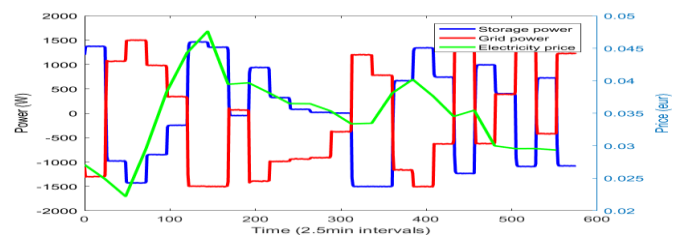
Fig. 2. EMS example of optimal power profiles for battery and grid
