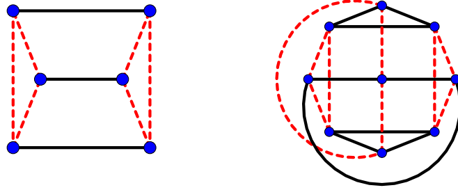
FIGURE 9. The possible orbits for two-dimensional Hadamard models with long steps in \{-2, -1, 0, 1\}^2 , depending on whether there are steps with -2 in only one coordinate (left) or both coordinates (right). The convention for dashed and solid edges is the same as in Figure 4.
