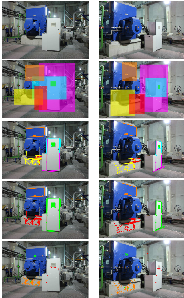
Fig. 1. Overview of our homographies estimation method. Row 1: Two views of an industrial environment. Row 2: Examples of matched regions (one color per match). Row 3: Inliers (points and segments) from homographies estimated between matched regions (one color per homography). Row 4: Inliers after merging homographies. Row 5: Inliers of the first three planes obtained by 4-points multi-RANSAC.
