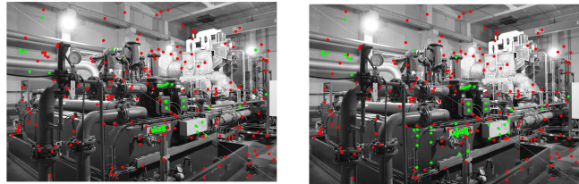
Fig. 3. Example of test images on which ORSA inliers (in green) are more numerous among our matches (right) rather than among LIFT ones (left).
