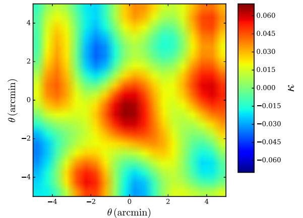
Figure 2. The stacked, weighted 2D \kappa profile recovered from the analysis of CMB temperature data around 3697 redMaPPer clusters. Each pixel in the cutout is 0.5 arcminutes on a side.
