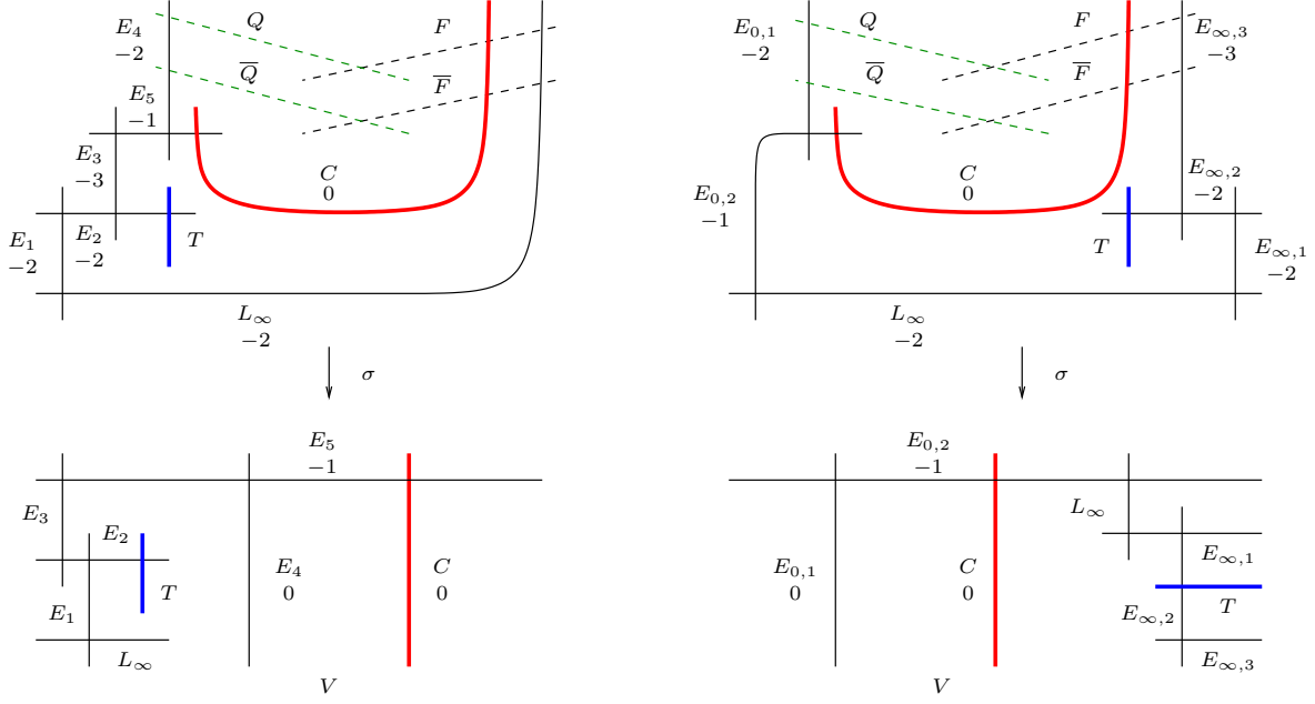
FIGURE 5.5. One singular point: case A_6 on the left and A_5^* on the right.
