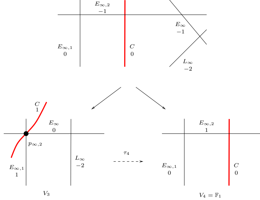
FIGURE 5.3. Three singular points, step 3: case A_2 + 2A_1^i or A_2 + 2A_2^i .
