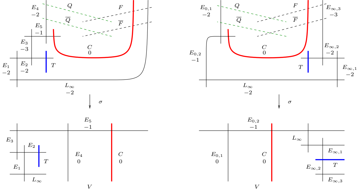
FIGURE 5.5. One singular point: case A_6 on the left and A_5^* on the right.
