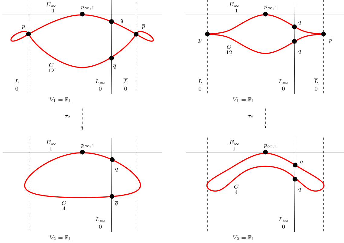
FIGURE 5.2. Three singular points, step 1: case A_2 + 2A_1^i on the left and A_2 + 2A_1^j on the right.
