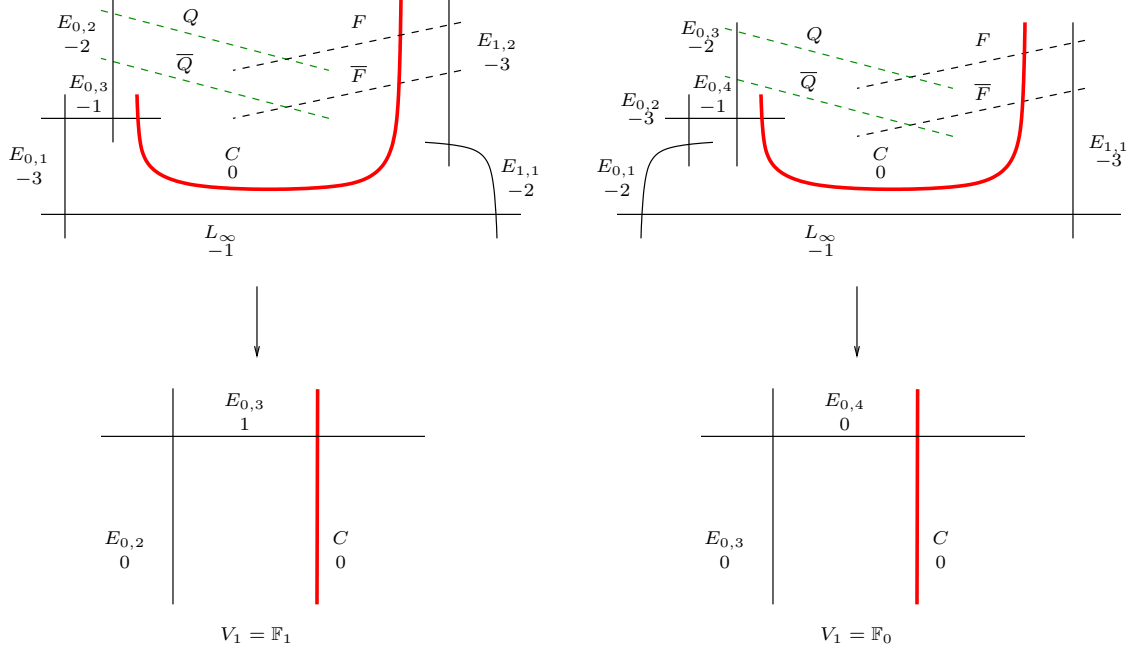
FIGURE 5.4. Two singular points: case A_2 + A_3^* on the left and A_4 + A_1^* on the right.
