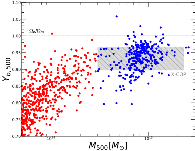
Fig. 2. Baryon depletion factor Y_b at R_{500} for the clusters in The300 simulation (filled circles). The blue points show the objects with a mass M_{500} > 3 \times 10^{14} M_\odot . The hashed grey shaded area shows the mass range covered by X-COP clusters and our determination of the universal baryon depletion factor and its scatter.
