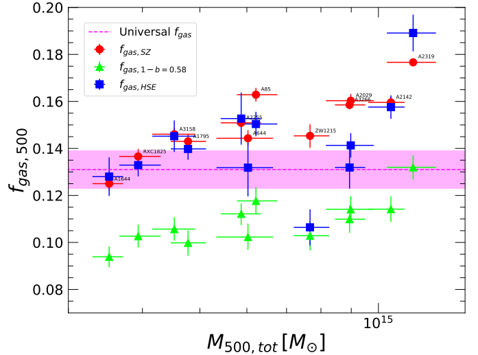
Fig. 6. Intracluster medium gas fraction at R_{500} obtained from our reference hydrostatic-based mass model (blue squares) as a function of the total mass corrected for non-thermal pressure support (see Sect. 4.3). The red points show the gas fraction obtained using the Planck PSZ2 masses estimated from the Y_{SZ} - M_{500} relation (Planck Collaboration XXVII 2016), whereas the green triangles show the gas fraction that would be obtained by correcting the PSZ2 masses with a uniform mass bias 1 - b = 0.58 \pm 0.04 (Planck Collaboration XXIV 2016). The dashed magenta line and shaded area represent the universal gas fraction estimated in Sect. 3.1.
