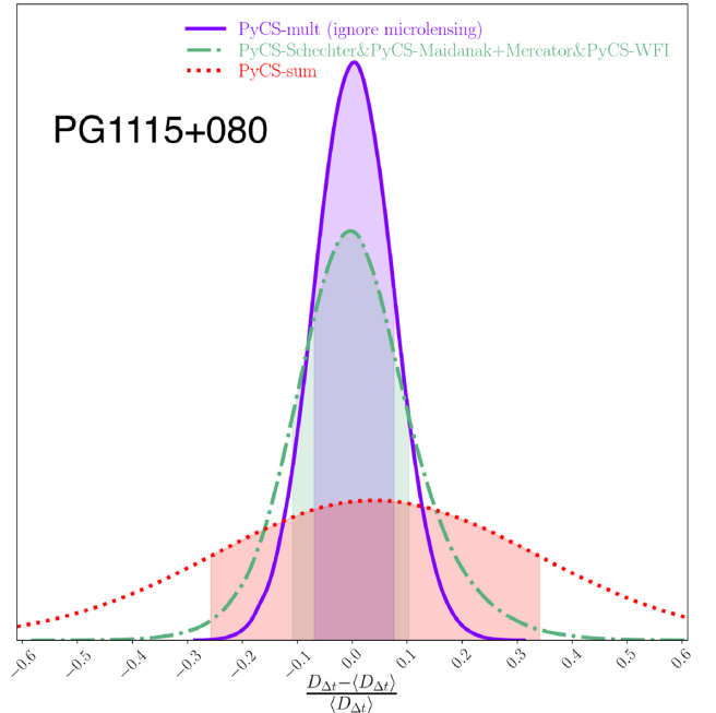
Figure 6. The comparison of the fractional difference of D_{\Delta t} among the case that ignores the microlensing time-delay effect (7.3 percent), the case that uses PyCS-Schechter&PyCS-Madanak+Mercator&PyCS-WFI (10.4 percent), and the case that uses PyCS-sum (30 percent). Note that the last two curves have already marginalized over all different accretion disc configurations. In the case of PG 1115+080, the uncertainty of D_{\Delta t} increases from \sim 7 percent to \sim 10 percent. The shaded regions and the percentages represent the 1\sigma uncertainties.
