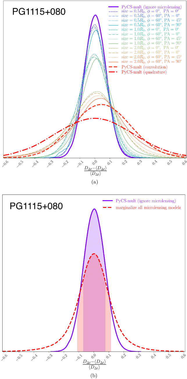
Figure 4. The fractional difference of D_{\Delta t} in different conditions. In panel (a), the top curve shows the case that ignores the microensing effect; the two curves at the bottom represent the cases in which we modify the PyCS-mult by convolving with the loosest case of microensing model and by adding the loosest case of microensing model in quadrature respectively, and the rest are the results with different accretion disc configurations. In panel (b), the top curve shows the case that ignores the microensing effect (7.3 per cent) and the bottom curve shows the constraint on D_{\Delta t} after we marginalize the different accretion discs listed in Section 2 (11.3 per cent). The shaded regions and percentages represent the 1\sigma uncertainties.
