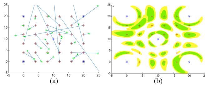
Figure 1: Node location (red crosses) estimates from RSS of waves emitted by anchors (blue stars). (a) Estimates and confidence regions from ML estimation (b) Confidence regions defined by LSCR
