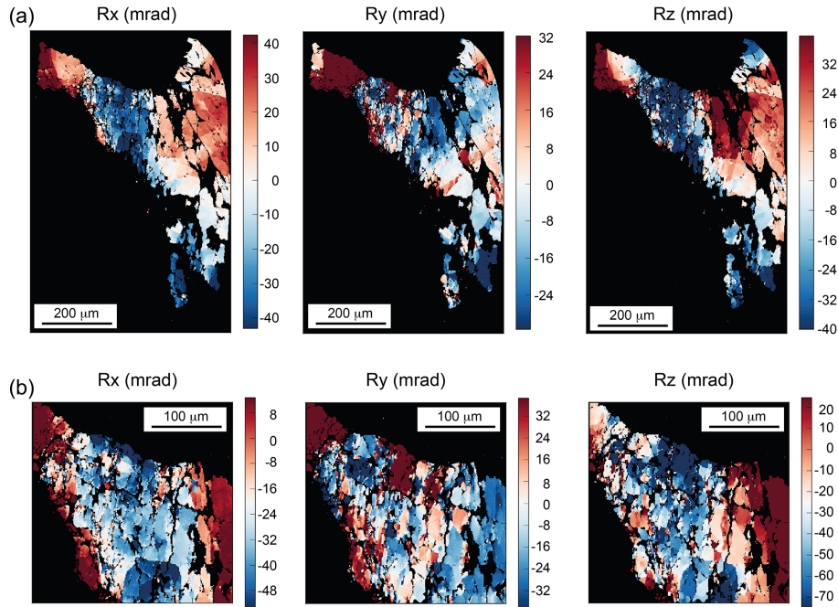
Figure 9. Maps of the R_x , R_y and R_z rotations of the crystal lattice around the x , y and z axes (sample referential), in the region explored in Fig. 8. R_x , R_y and R_z were calculated with LaueTools from the EBSD data of Fig. 8. The x , y map positions and the Euler angles of the EBSD file were first transformed in order to adapt to the LaueTools (LT) reference frames. The corresponding transformations are described in Sect. S1. Histograms of orientation matrix components were then built for different rectangular regions in the map of Fig. 8a in order to identify the frequency peaks associated with the blue crystallite in the center of the map and to define the thresholds for selecting the map points belonging to this crystallite according to their crystallographic orientation. In Fig. 9a, all the non-black pixels have their \mathbf{a}^* vector within less than 245 mrad ( 14^\circ ) of the x axis. These pixels were used to calculate the mean orientation matrix of the crystallite (used as the zero for rotations). The twinned regions appear in black, i.e., they were excluded from the crystallite. (a) Rotation components for the right part of Fig. 8a. (b) Zoom on the top-center area of Fig. 8a. Scales in milliradians differ (in amplitude and offset) among the different maps in order to enhance the contrast for each rotation component.
