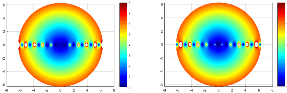
FIGURE 8. Plots of |\Lambda_{\mathfrak{D}}(\omega)| (left) and |\Lambda_n(\omega)| (right), for |\omega| < 2\pi , \alpha = \mu = 0.6
