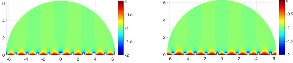
FIGURE 9. Plots of \text{Im}(\omega^{-1}\Lambda_\delta(\omega)) (left) and \text{Im}(\omega^{-1}\Lambda_n(\omega)) (right), for |\omega| < 2\pi , \alpha = \mu = 0.6 . Remark that \omega^{-1}\Lambda_\delta(\omega) has a pole in \omega = 0 , unlike \omega^{-1}\Lambda_n(\omega) .
