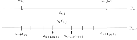
FIGURE 5. Inductive construction of the mesh \Gamma_n
