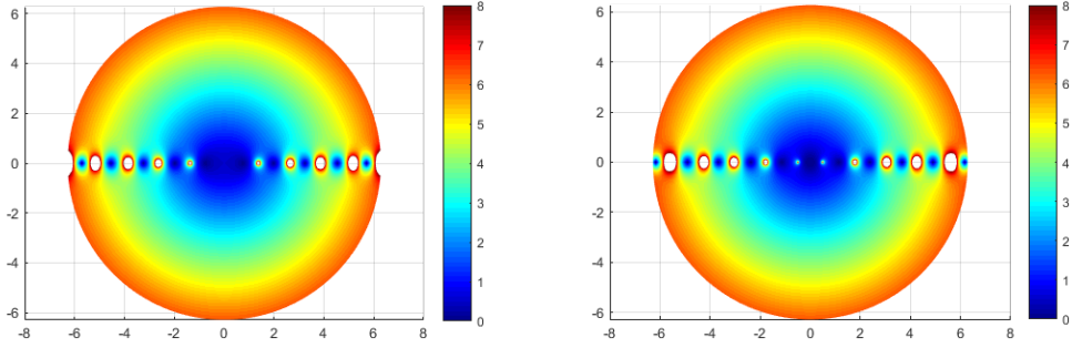
FIGURE 8. Plots of |\Lambda_\delta(\omega)| (left) and |\Lambda_n(\omega)| (right), for |\omega| < 2\pi , \alpha = \mu = 0.6
