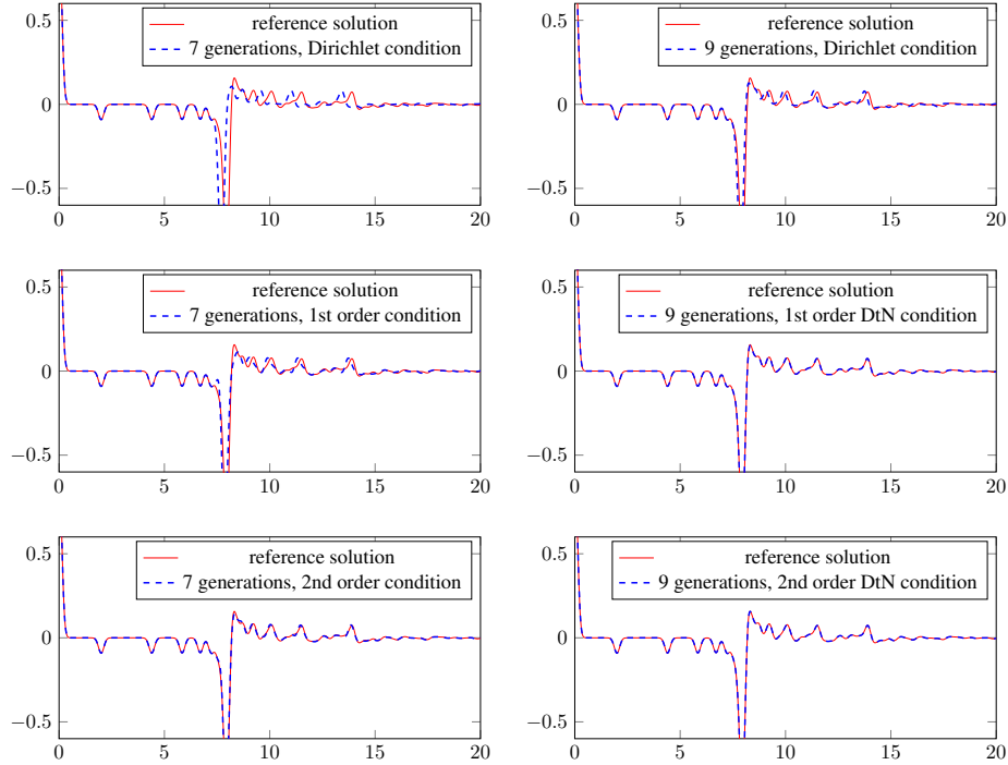
FIGURE 11. Left row: the dependence of u(M, t) on time for the exact (red solid line) and the truncated tree on 7 generations (blue dashed line). Top: Dirichlet condition. Middle: the first order DtN condition. Bottom: the second order DtN condition. Right row: the dependence of u(M, t) on time for the exact (red solid line) and the truncated tree on 9 generations (blue dashed line). Top: Dirichlet condition. Middle: the first order DtN condition. Bottom: the second order DtN condition.
